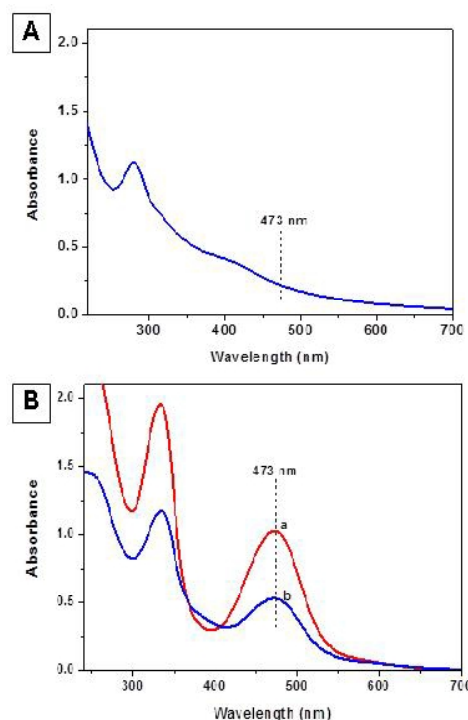
Fig. 6 (A) UV-vis spectra of PDA, (B) rifampicin before (a) and after (b) the drug loading
