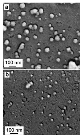
Fig. 1 SEM image of (a) PDA and (B) PDA-R
