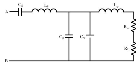
Fig. 7 Diagram of Matching Network
