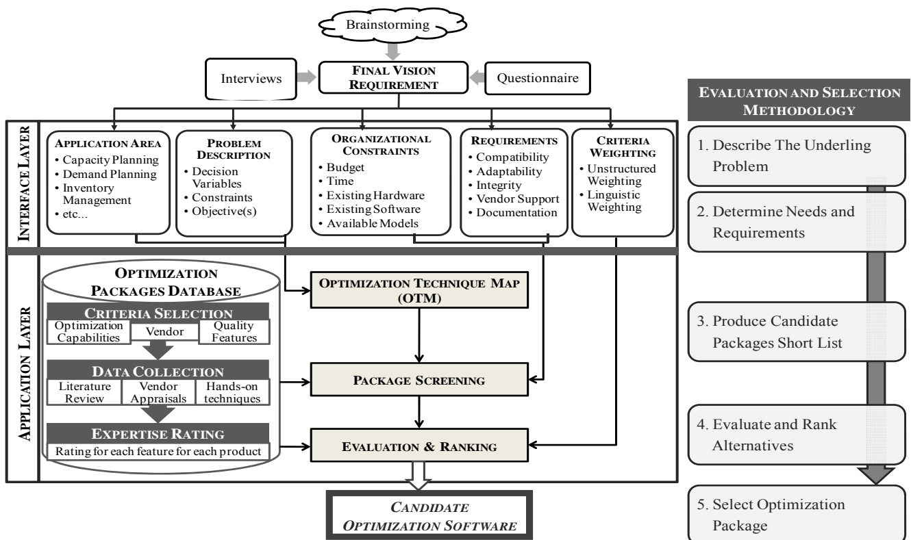
Fig. 1 The proposed framework for optimization software selection
