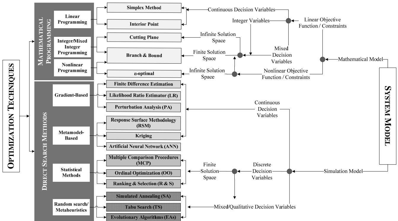
Fig. 2 Optimization Techniques Map (OTM)
