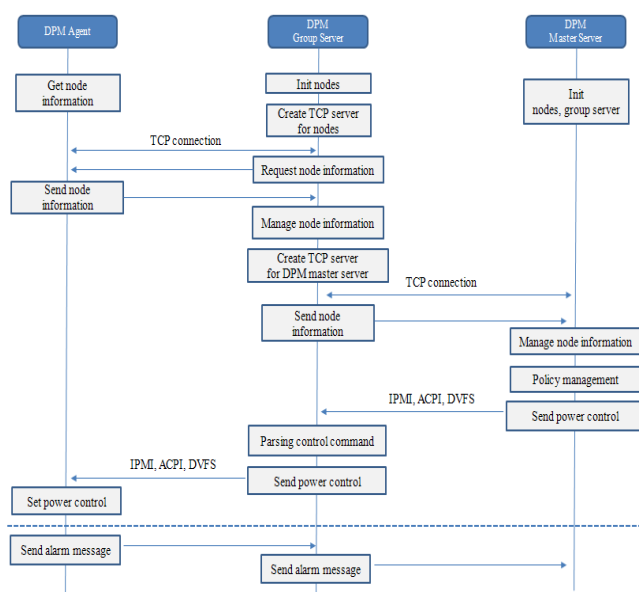
Fig. 4 DPMS flow chart
