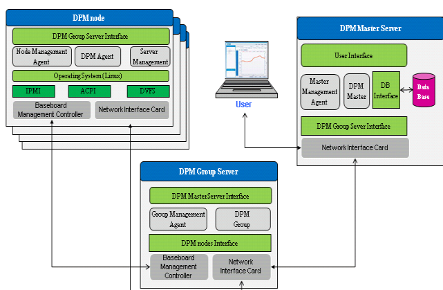
Fig. 3 DPMS block diagram
