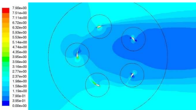
Fig. 13 Contours of absolute velocity [m/s] for the whole rotor area; bare rotor configuration, \lambda = 2.16 , \theta = 90^\circ
