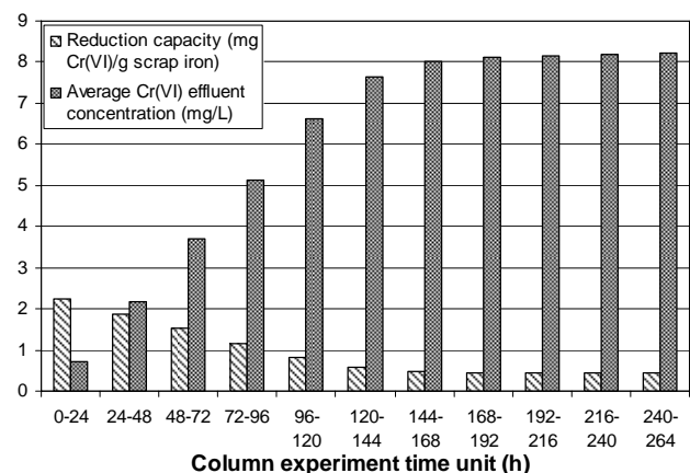
Fig. 4 Scrap iron reduction capacity ( RC_{SI} ) and average Cr(VI) effluent concentration vs. time, at feed solution pH = 5.1
