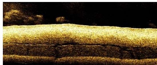
Fig. 7 2-MHz Sonar data before correction
