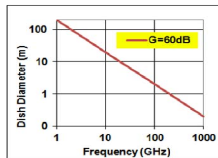
Figure 5. Reflector antenna diameter versus frequency.
