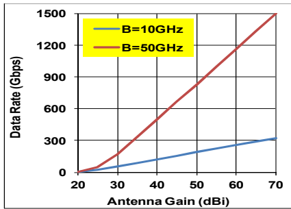
Figure 8. The maximum achievable data rates for interior WLAN applications with 10 and 50 GHz channel bandwidths.
