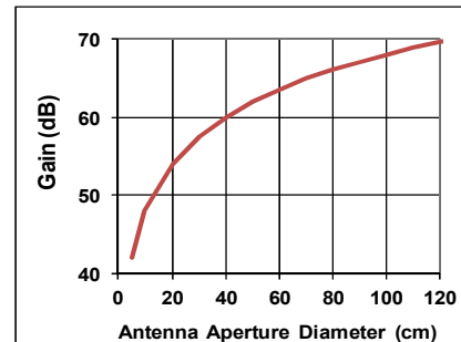
Figure 12. Antenna gain versus aperture size at 0.5 THz.
