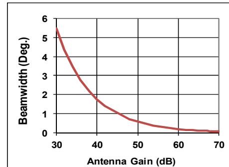
Figure 4. Antenna half-power beamwidth versus antenna gain.
