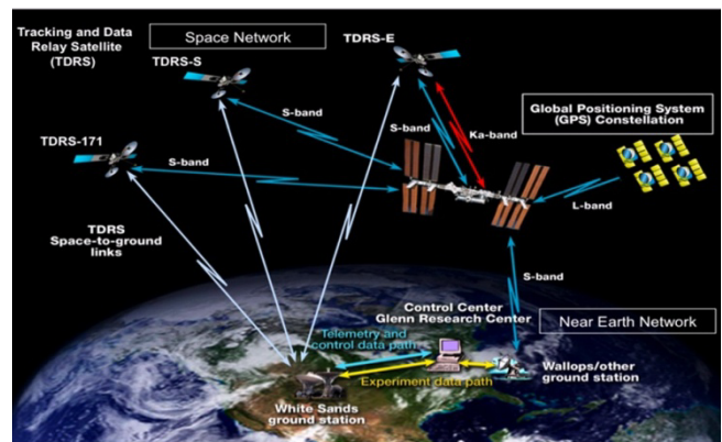
Figure 2. The current communication systems for human spaceflight missions at S-band, Ku-band, and Ka-band.
