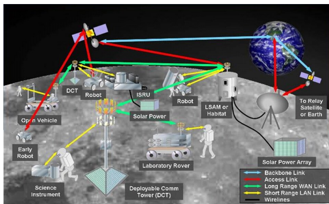
Figure 9. Surface communication network architectures for the future human space exploration missions [16].
