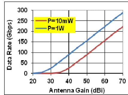
Figure 10. The maximum achievable data rates for the planet surface wireless applications with 10 mW and 1 W transmit power.
