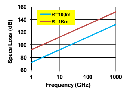
Figure 3. Free space propagation loss versus frequency.
