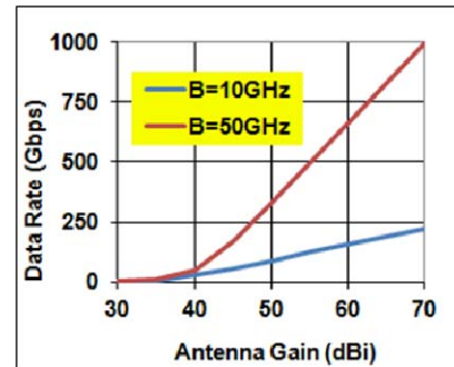
Figure 11. The maximum achievable data rates for planet surface applications with 10 and 50 GHz channel bandwidths.
