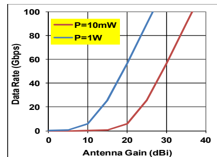
Figure 7. The maximum achievable data rates for the interior WLAN applications with 10mW or 1W transmit power.
