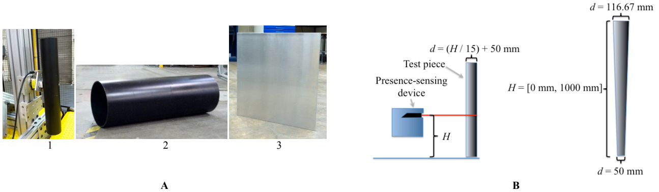
Fig. 1. Current test pieces used by the AGV (A) and industrial robot (B) standards. (A) shows the 1) vertical (shown being used for measuring bumper force), 2) horizontal, and 3) flat plate test pieces with their proper coatings. (B) shows the range of artifact radii as a function of the detection zone height.
