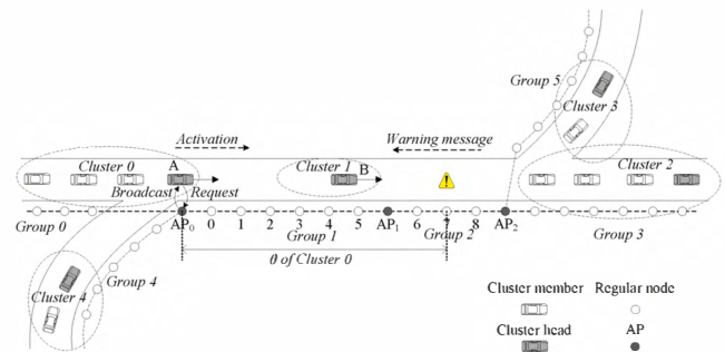
Figure 2. Network Deployment
