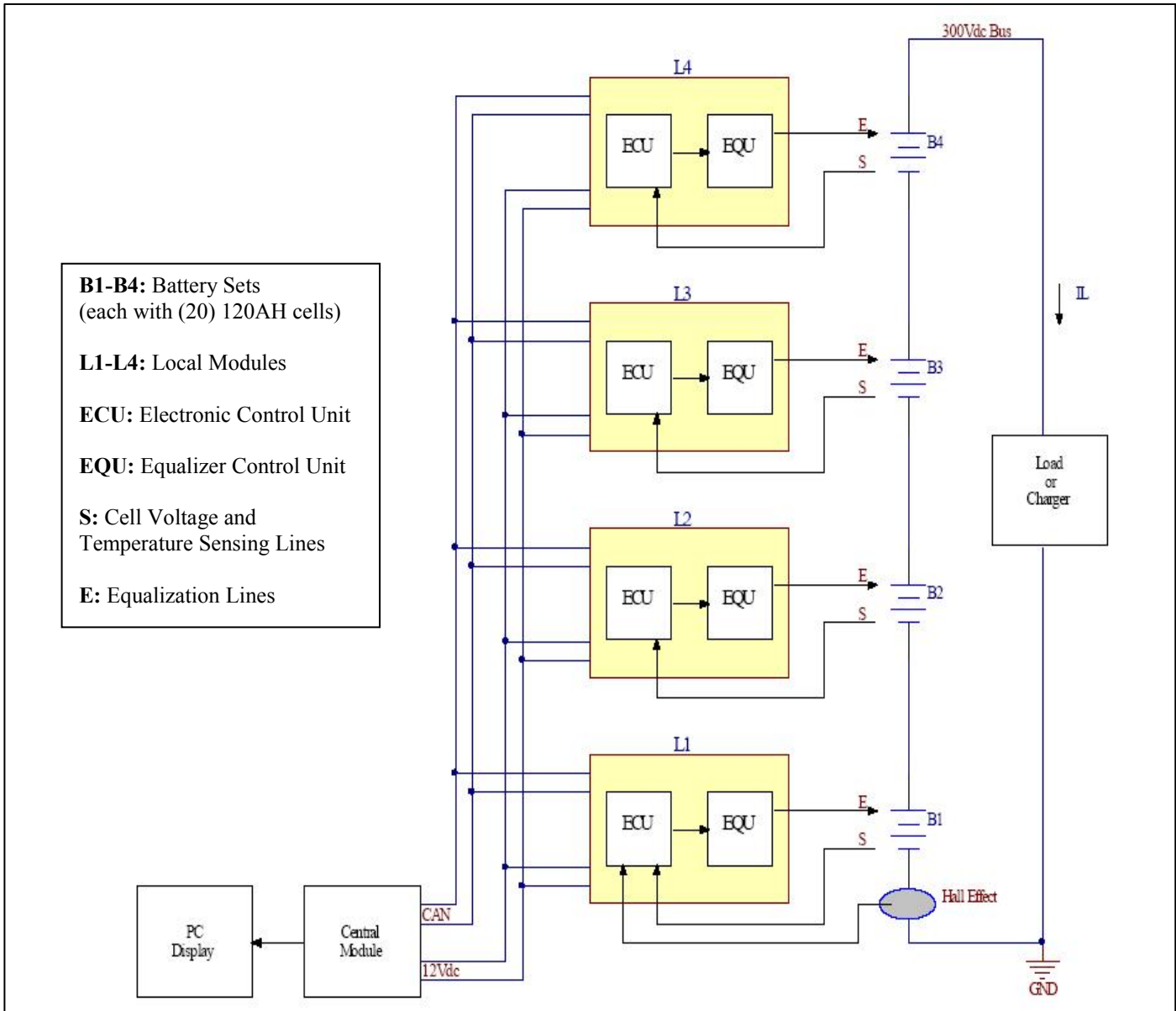
Figure 4. Modularized Battery Stack and BMS with Four Locals
