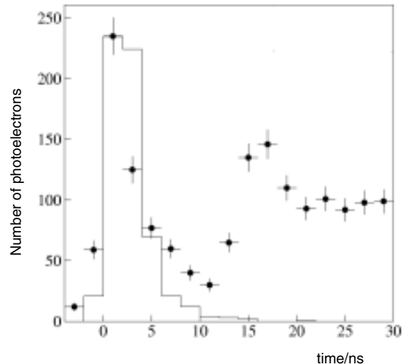
Fig. 5. Light yield from simulated delta rays: Monte Carlo is represented by the smooth line, the data by the dots. Delta rays are the dominant component in the first background photon peak.
