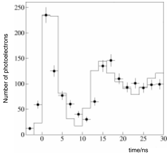
Fig. 6. Time distribution of photon background pulses in the first 30 ns. The data (a combination of both the mirror and photon trap data) is represented by the dots and the Monte Carlo by the smooth line. The Monte Carlo was normalized to the data using a factor of 0.6.
