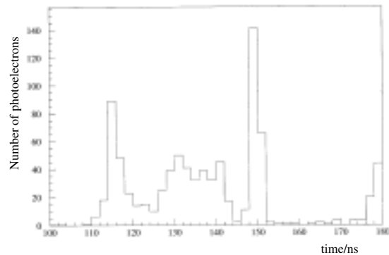
Fig. 3. Measured time distribution of photon pulses obtained from the peak finding algorithm using the mirror data. The Cherenkov signal arrives at channel 150. The hits before this time are all considered background.
