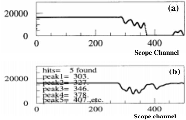
Fig. 2. Digital scope output from a single event for the mirror setup (a) and the photon-trap setup (b). The horizontal axis is time in terms of scope channels (1 scope channel = 0.4 ns ) and the vertical axis is the amplitude. In (a) one notices the large Cherenkov pulse arriving at channel 375 and the background pulses arriving earlier. In (b) there is a distinct lack of the large Cherenkov pulse. The background pulses fade away as one approaches 70ns. (The text is the output of the peak finding algorithm displaying the location of each photon hit)
