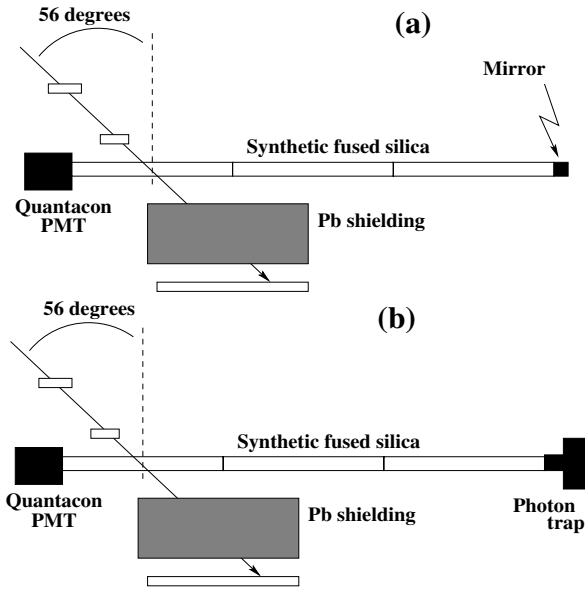
Fig. 1. Experimental setups used to study the photon background. The Cherenkov signal propagates to either (a) the mirror or (b) the photon trap. In the former case, a window of \sim 36 ns is available to study the early photon background activity before the Cherenkov signal returns; in the latter case a \sim 70 ns window is available.
