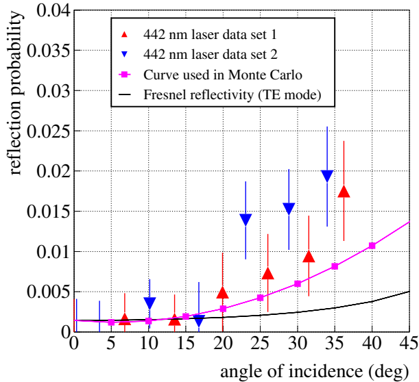
Fig. 4. The Fresnel curve is based on the measurement of the index of refraction. Also shown is the data from two different measurements of the reflectivity per bounce from the glue/silica interface. Finally, the curve with square references is used in the Monte-Carlo program that simulates the 4m long bar cosmic ray experiment mentioned in section 2.
