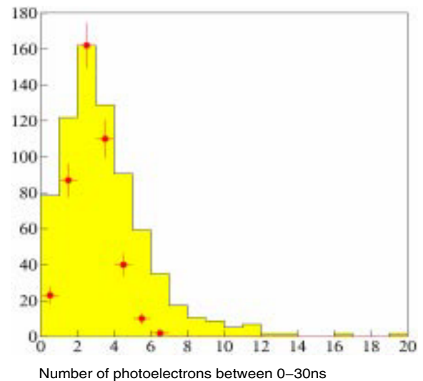
Fig. 8. Multiplicity distribution of background photons for the mirror setup (30 ns), Data (dots) and Monte Carlo (histogram) agree well in terms of the most probable number 3.
