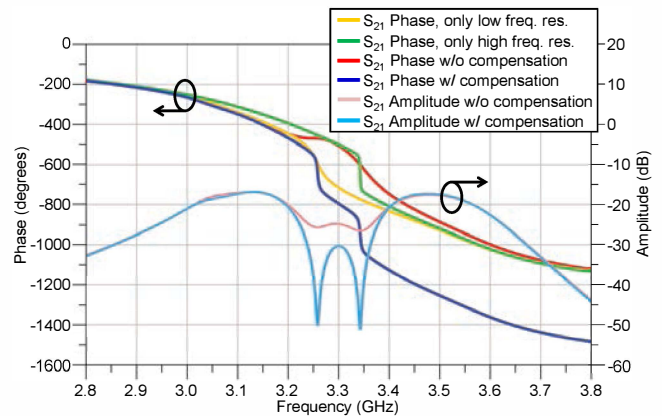
Fig. 3. The phase and corresponding amplitude of S_{21} with and without compensation for proximity of the resonances.
