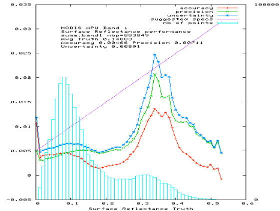
Figure 2a: APU for the MODIS red band, Collection 5.
