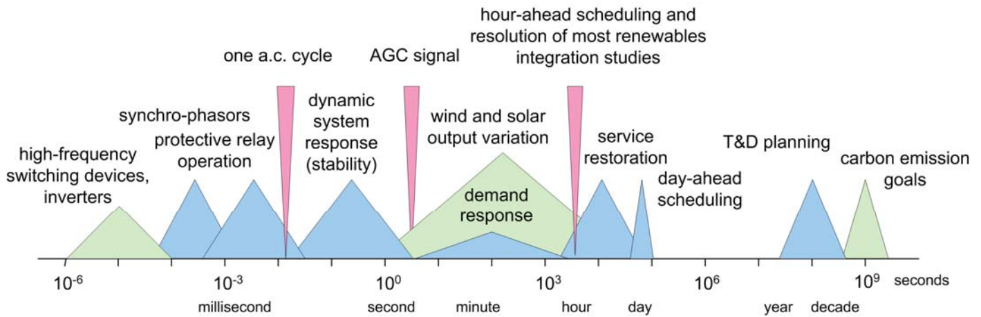
Figure 1. Time scales in electric grid operation.
