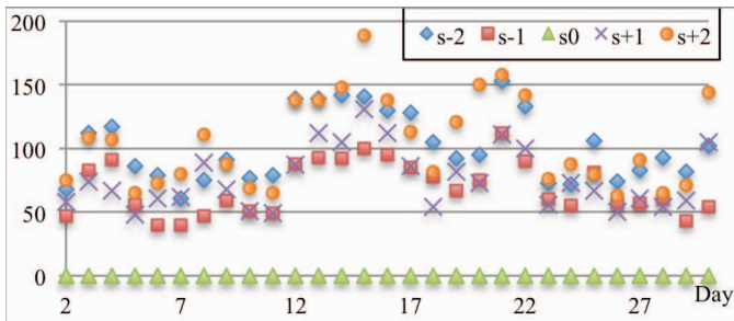
Fig. 17. Number of conflicts for 29 days after conflict resolution under “s0” wind forecast scenario evaluated over 5 wind forecast scenarios
