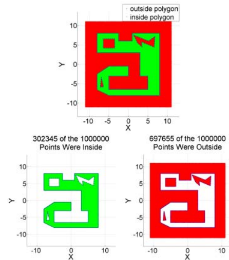
Figure 6. Monte Carlo Evaluation of Boundary Violation Function.
