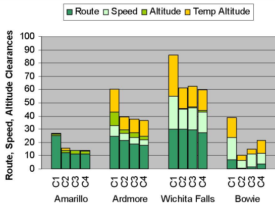
Figure 13. Number of Route, Speed, and Altitude Clearances
