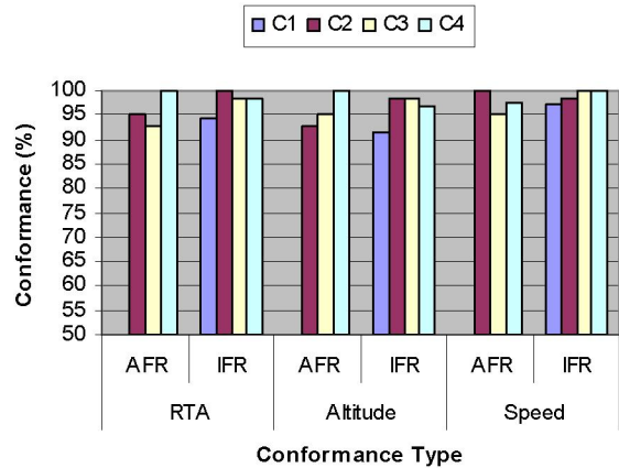
Figure 14. RTA, Altitude, and Speed Conformance at the BAMBE Meter Fix
