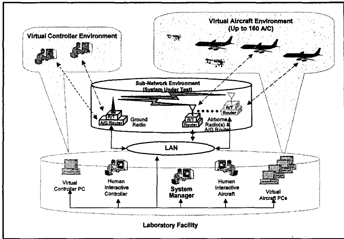
Figure 1. GRC's Communications Emulation Testbed
