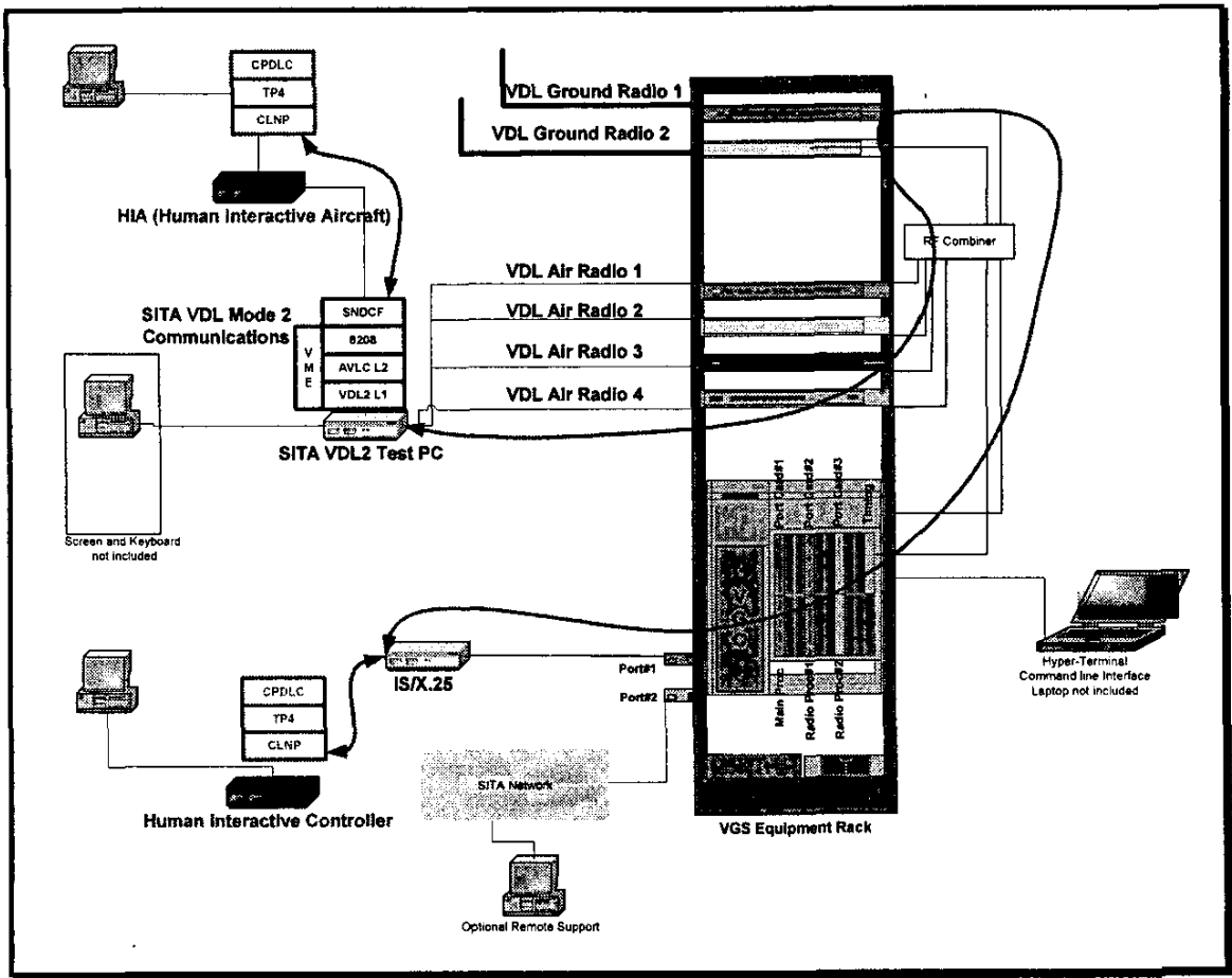
Figure 6. VDL Mode 2 Communications Equipment
