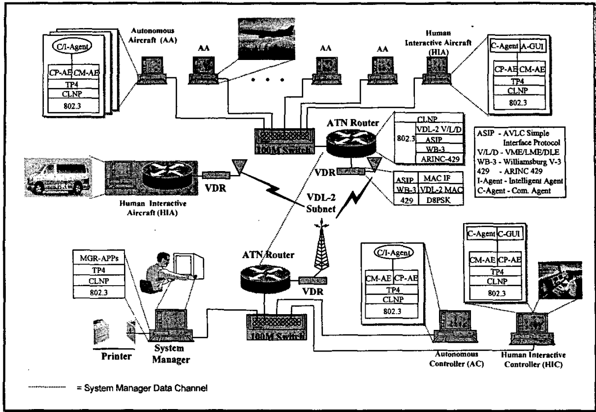
Figure 2. CM and CPDLC Communications Architecture
