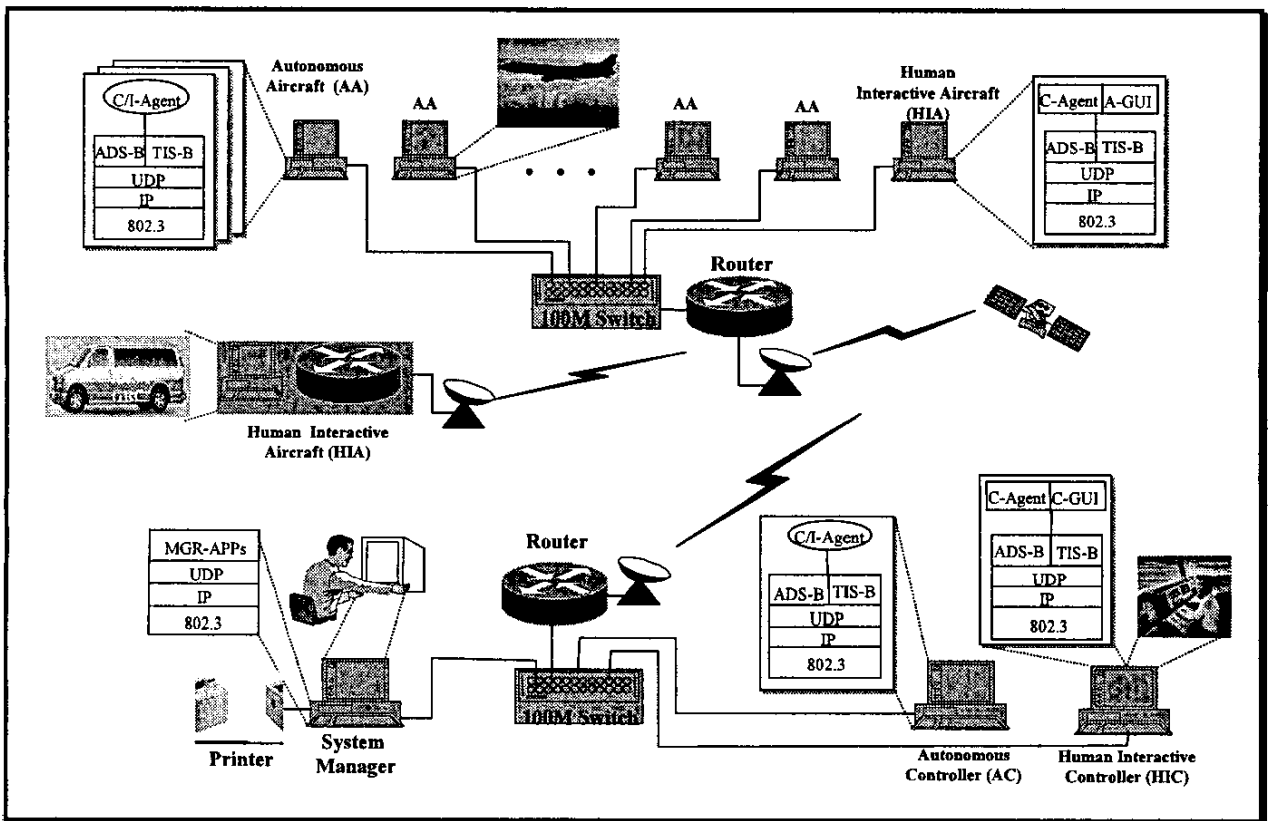
Figure 7. ADS-B/TIS-B Communications Architecture
