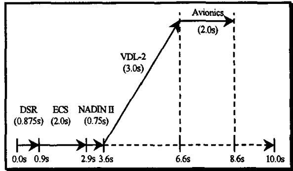
Figure 5. Mean Transfer Delay Time Budgets
