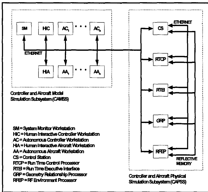
Figure 8. VAC Testbed with the JCS
