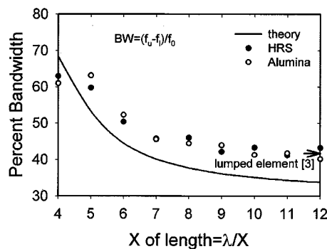
Fig. 4. Measured and theoretical bandwidth of miniaturized Wilkinson dividers fabricated on HRS and alumina.
