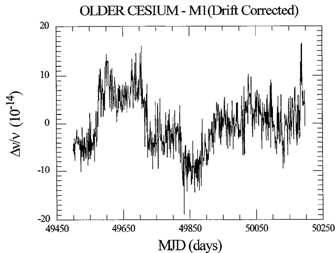
Fig. 2. Normalized frequency difference between an older generation high performance cesium standard and maser M1.
