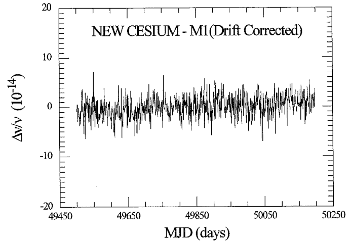
Fig. 3. Normalized frequency difference between a new generation high performance cesium standard and maser M1.
