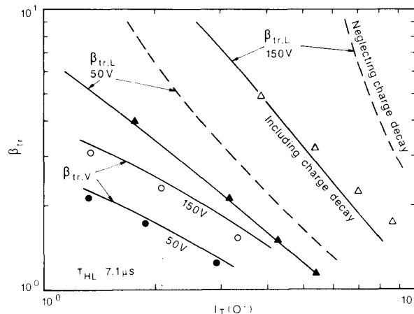
Fig. 12. Comparison of theoretical (solid curves) and measured ( \circ \bullet \triangle \blacktriangle ) values of \beta_{tr} versus current for both constant anode supply voltage switching and clamped inductive load switching at 50 V and 150 V for 7.1- \mu s device. Dashed curves are the calculated values of \beta_{tr,L} neglecting decay of charge during voltage transition.
