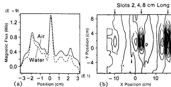
Figure 4. (a) Relative response of SQUID sensor to slotted steel plate in air and under water; (b) magnetic field contour map for plate with 3 slots. (Reference 5)
