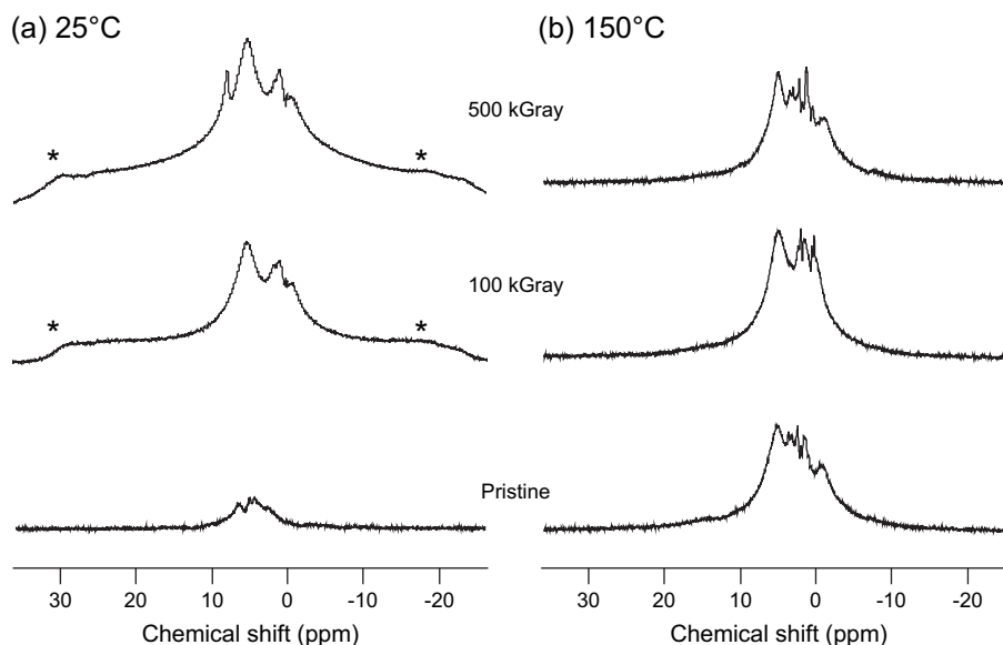
Fig. 5. ^1\text{H} MAS NMR spectra of FPC-461 irradiated to 0, 100, and 500 kGy in nitrogen at (a) 25 °C, spinning at 12 kHz and (b) 150 °C, spinning at 4.5 kHz. Spinning sidebands are indicated by a star (*).
