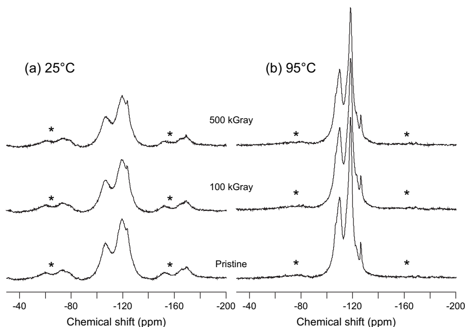
Fig. 8. ^{19}\text{F} MAS NMR spectra of FPC-461 irradiated to 0, 100, and 500 kGy in nitrogen at (a) 25 °C and (b) 95 °C. Both experiments were performed at 17 kHz MAS speeds. Spinning sidebands are indicated by a star (*).
