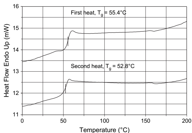
Fig. 1. DSC curves for pristine FPC-461. The curve for the first heat has been vertically shifted by 2 mW. The glass transition temperatures on each curve are noted with a tic mark.
