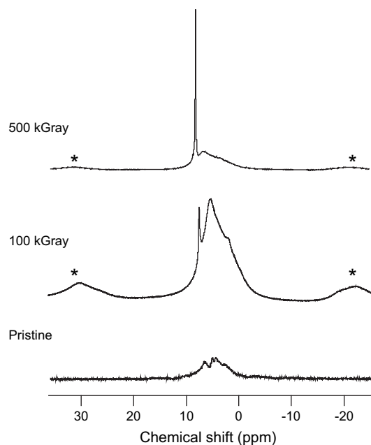
Fig. 2. ^1\text{H} MAS NMR spectra of FPC-461 irradiated to 0, 100, and 500 kGy in air at room temperature with MAS speeds of 13 kHz. Spinning sidebands are indicated by a star (*).
