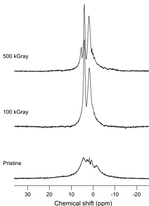
Fig. 4. ^1\text{H} MAS NMR spectra of FPC-461 irradiated to 0, 100, and 500 kGy in air at 150 °C with MAS speeds of 4.5 kHz.
