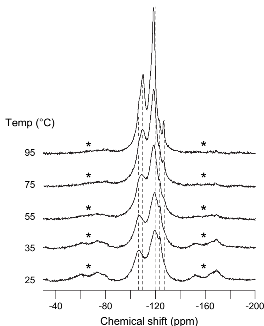
Fig. 6. Variable temperature ^{19}\text{F} MAS NMR spectra of FPC-461 irradiated to 500 kGy in air. The spectra were obtained under MAS conditions at 17 kHz spinning speeds. Spinning sidebands are indicated by a star (*).
