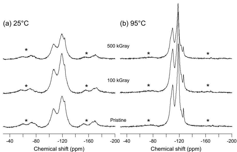
Fig. 7. ^{19}\text{F} MAS NMR spectra of FPC-461 irradiated to 0, 100, and 500 kGy in air at (a) 25 °C, and (b) 95 °C. Both experiments were performed at 17 kHz MAS speeds. Spinning sidebands are indicated by a star (*).
