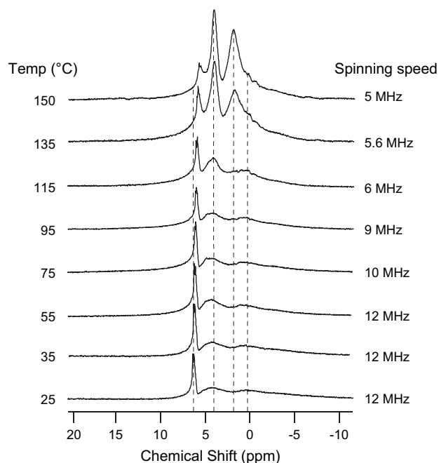
Fig. 3. Variable temperature ^1\text{H} NMR spectra of FPC-461 irradiated to 500 kGy in air. The spectra were obtained under MAS conditions at the spinning speeds indicated at the side.
