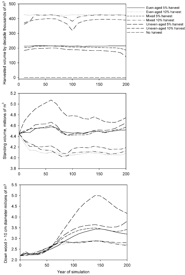
Fig. 7. Estimated volume of harvested timber, residual standing timber, and down wood under seven simulated forest management scenarios in southern Missouri.
