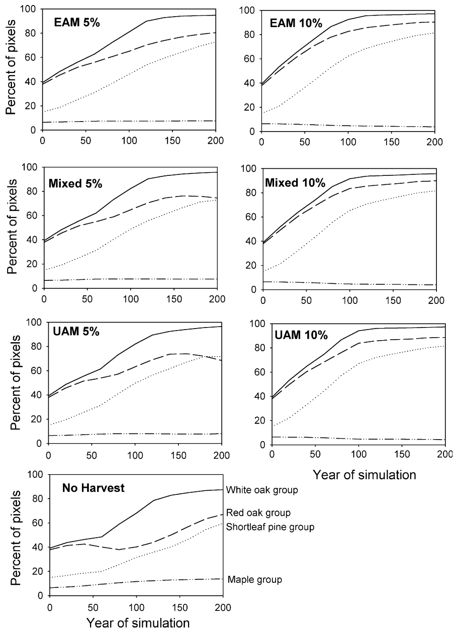
Fig. 6. Percent of pixels where a tree species group is present (regardless of age) under seven simulated forest management scenarios in southern Missouri. We populated the initial landscape (year 0) with one species per 0.09 m pixel. Over time the number of species on most sites increased to two or more through simulated regeneration, succession, and response to disturbance. Hence, as the simulations progressed species in the black oak, white oak, and pine groups were each present across 60 to >90% of the landscape.
