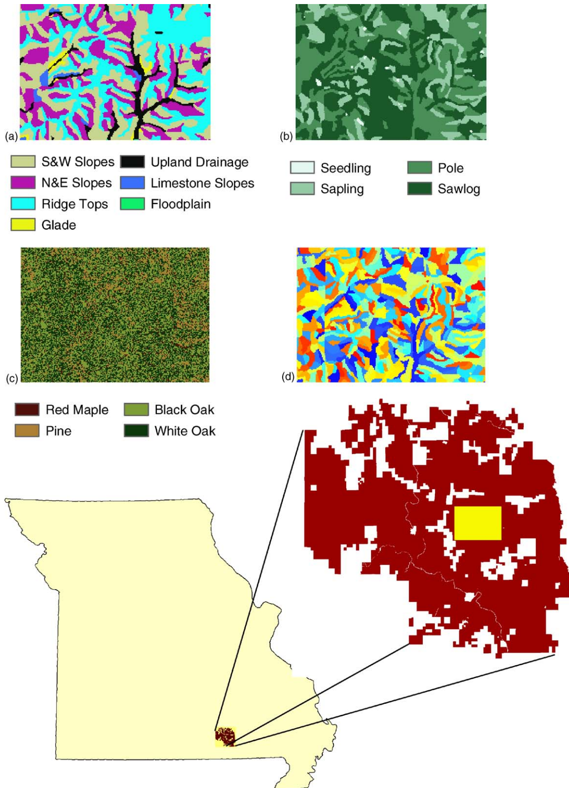
Fig. 1. Location of the landscape used to simulate forest management scenarios in southern Missouri and enlargement showing initial (a) land types, (b) size classes, (c) dominant species, and (d) stand boundaries. Pixel size is 30 m by 30 m (0.09 ha).
