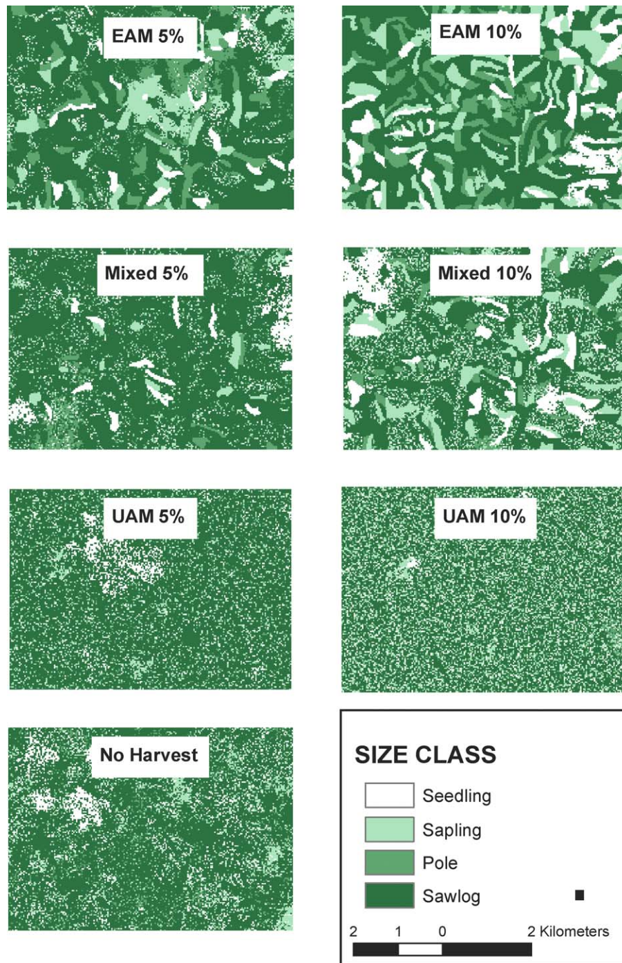
Fig. 3. Spatial arrangement of forest size classes at simulation year 200 for seven forest management scenarios on a 2835 ha subset of the 71,142 ha landscape in southern Missouri. Individual pixels are 30 m by 30 m (0.09ha).
