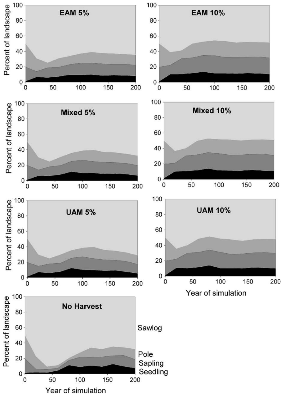
Fig. 2. Tree size class distribution by decade over 200 years of simulation of seven forest management scenarios in southern Missouri. Size classes are groupings of the 10-year age classes modeled by LANDIS: seedling \leq 10 years; sapling = 20, 30 years; pole = 40, 50 years; sawlog \geq 60 years.
