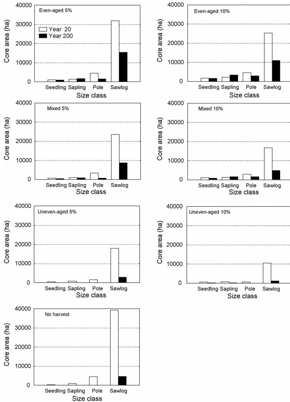
Fig. 5. Core area by size class in simulation year 20 (white bars) and 200 (shaded bars) under seven forest management scenarios in southern Missouri. Core area is the total area by size class (seedling, sapling, pole, or sawlog) that is at least 60 m from an edge boundary between any two adjacent size classes.
