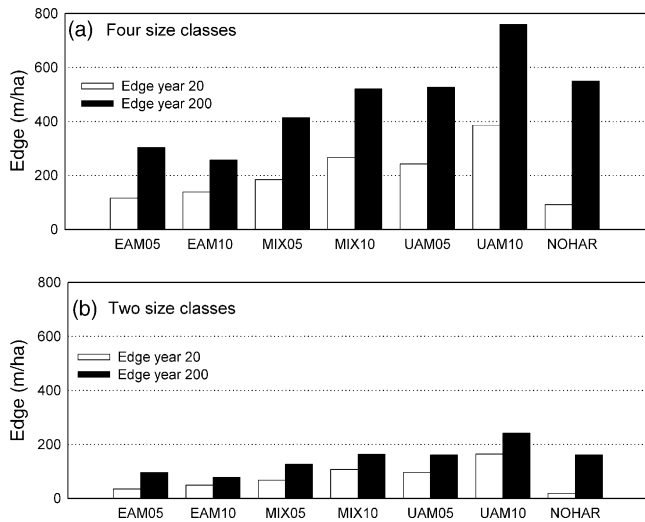
Fig. 4. Edge density (m/ha) under seven forest management scenarios in simulation year 20 and 200. In panel (a) edge was defined as the length of boundary between any two different size classes (e.g., seedling vs. sapling, seedling vs. pole, pole vs. sawlog, etc.). In panel (b) edge was defined as the edge between regeneration openings (seedling or sapling size class) and closed canopy forest (pole or sawlog size classes).
