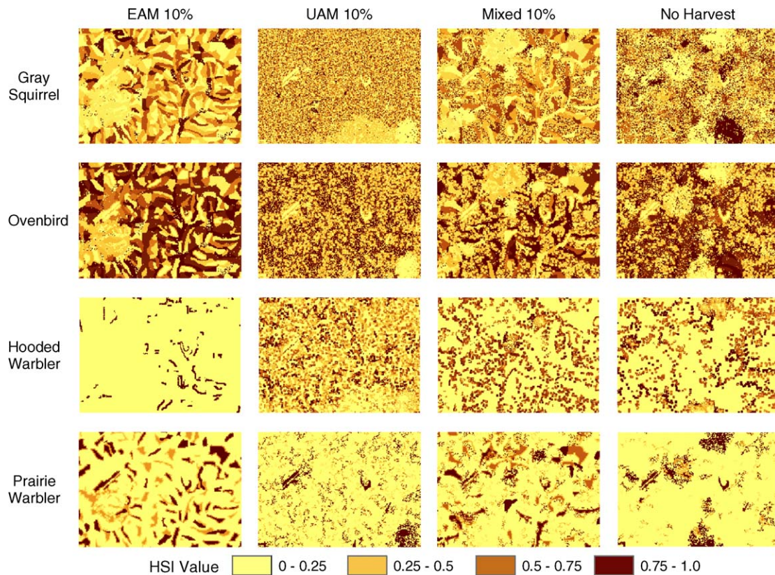
Fig. 8. Habitat suitability at year 200 for four wildlife species under four forest management scenarios on a 2835 ha subset of the 71,142 ha landscape for which we simulated landscape change. Habitat suitability ranges from 0 to 1 with 1 being optimal habitat.
