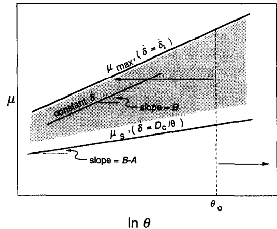
Fig. 1. Plot of friction coefficient against state, \theta . Lines of constant slip speed and \mu_{\max} , which is defined at \dot{\delta} = \dot{\delta}_i , have slope B . The steady-state friction, \mu_s , has the slope B - A . At stresses below \mu_s , \theta evolves to the right, increasing the strength of the fault at any reference slip speed. At stresses above \mu_s , \theta evolves to the left, decreasing the strength. Note that \mu_s and \mu_{\max} change as \theta evolves. The shaded portion of the graph schematically represents the region where the simplifying assumption employed for the simple patch solution, discussed below, is valid.
