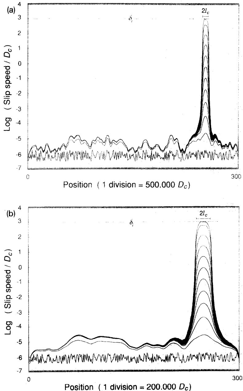
Fig. 5. Numerical model with 300 nodes and randomized normal shear stress and uniform initial shear stress. Parameters for the calculations are: A = 0.005 , B = 0.008 , \theta = 10^9 s, G = 10^4 \sigma , \dot{\tau} = 0 , uniform initial shear stress of (\mu_0 + 0.095)\bar{\sigma} and normal stress from \sigma = 0.95\bar{\sigma} to \sigma = 1.05\bar{\sigma} , where \bar{\sigma} is the mean normal stress. The logarithm of slip speed for faults with different values of D_c is indicated.
