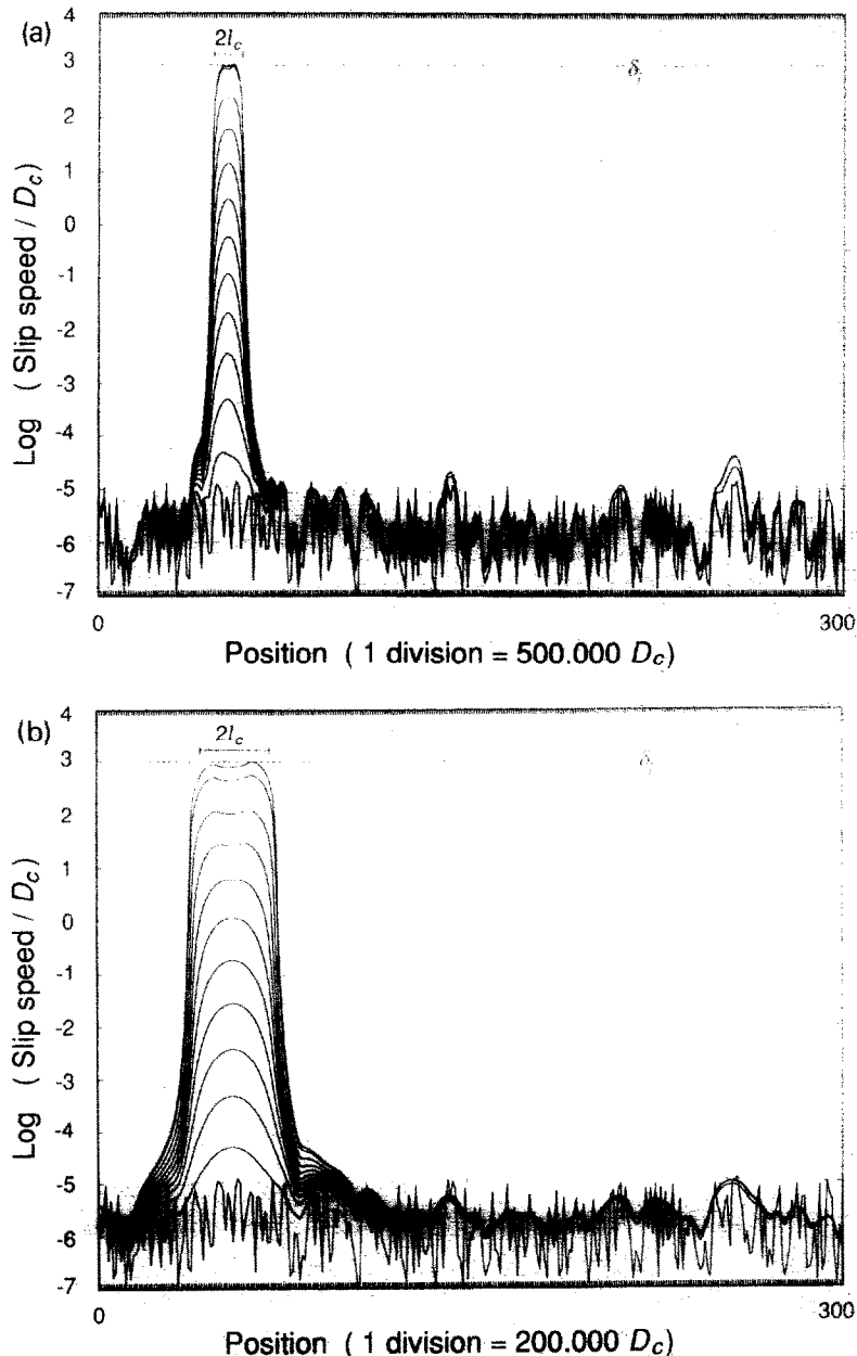
Fig. 4. Numerical model with 300 nodes and randomized initial shear stress. Parameters for the calculations are: A = 0.004 , B = 0.006 , \theta = 10^9 s, G = 10^4 \sigma , \tau = 0 , and initial shear stress from (\mu'_0 + 0.06)\sigma to (\mu'_0 + 0.08)\sigma . The logarithm of slip speed for faults with different values of D_c is indicated.
