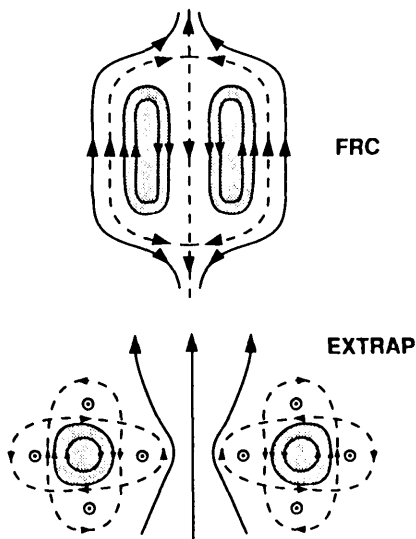
FIG. 11. Comparison of the FRC and Extrap geometries [169].
