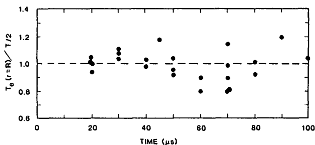
FIG. 23. Ratio of measured electron temperature T_e to the calculated half-pressure balance temperature T/2 as a function of time [276].
