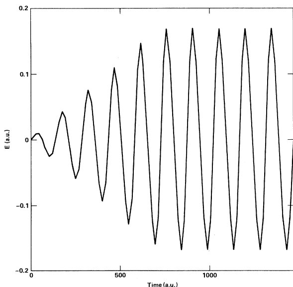
FIG. 2. Time evolution of the classical field strength for a photon wavelength of 1.064 \mu\text{m} and a rise time of five periods. Time is in atomic units ( 2.4189 \times 10^{-17} s).
