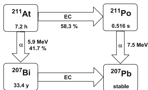
Fig. 4 Decay scheme of ^{211}\text{At}
