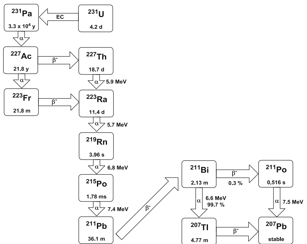
Fig. 6 Decay scheme of ^{223}\text{Ra} and ^{227}\text{Th}
