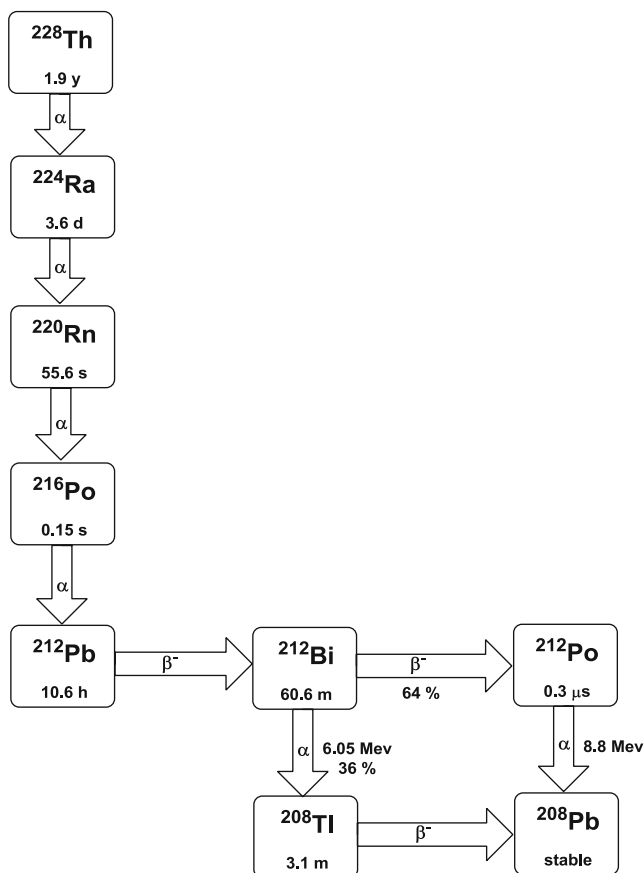
Fig. 5 Decay scheme of 212 Bi and 212 Pb
