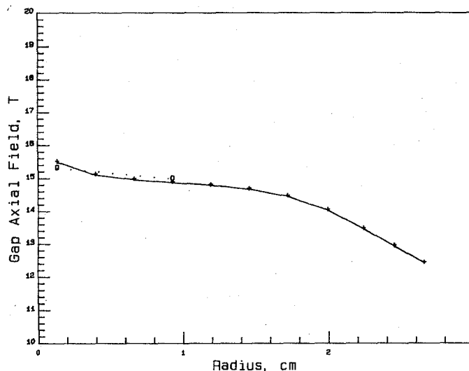
Fig. 4. Calculated axial field uniformity (solid line) vs experimental measurements (dotted line).
