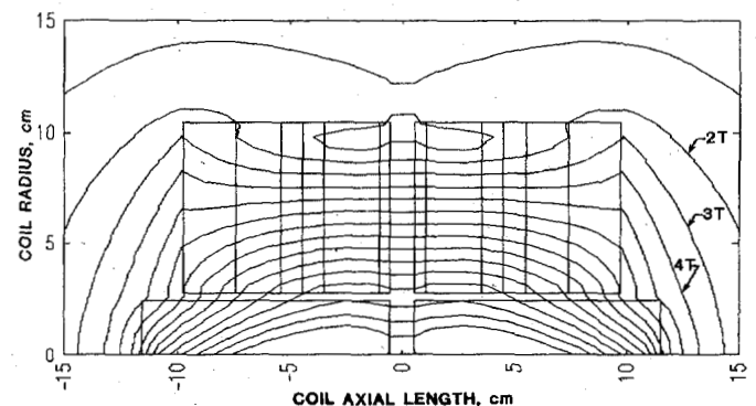
Fig. 2. Field contours of a commercially available tape magnet with holmium pole inserts.
