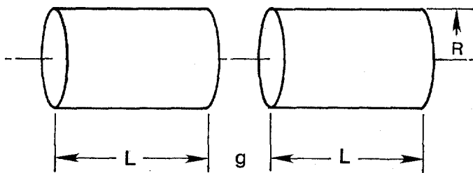
Fig. 3. Geometry of the two holmium cylinders. Note that R is radius, L is length, and g is gap.
