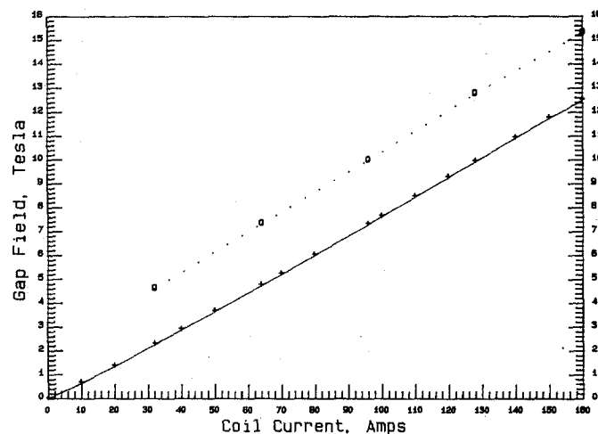
Fig. 5. Comparison of magnetic field vs current of the typical tape magnet (solid line) to the magnet with holmium poles (dotted line).
