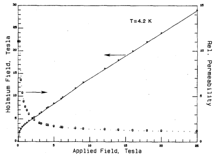
Fig. 1. Comparison of the magnetization curve (solid line) for rare earth element holmium to its relative permeability (dotted line).
