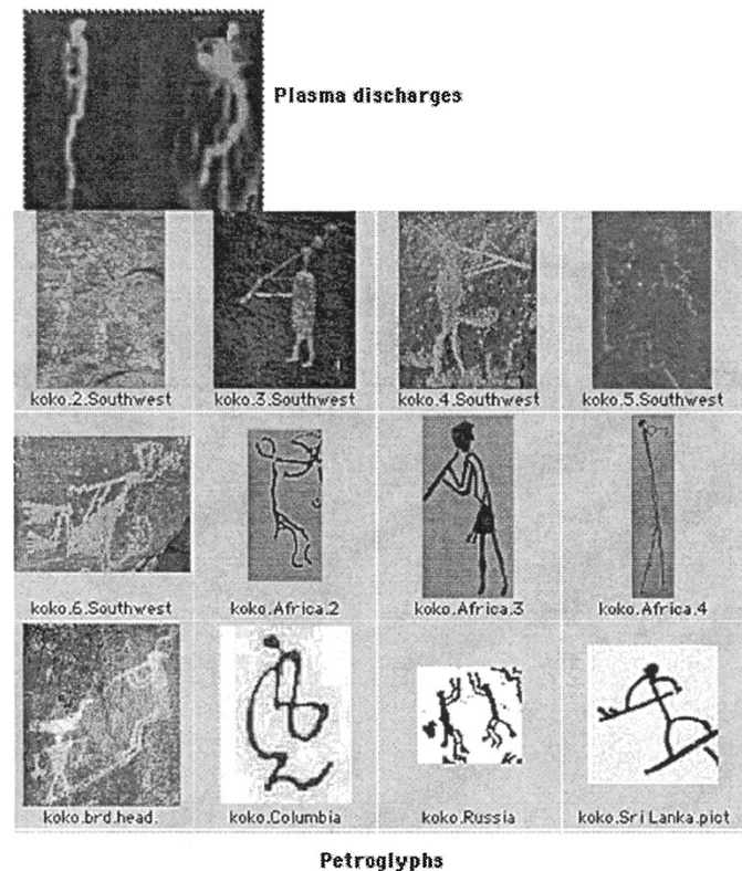
Fig. 37. Kokopelli. Examples from plasma discharges and world-wide interpretations on rock.
