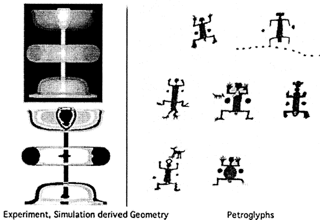
Fig. 32. (Left) Configuration and cross-sectional views of the intense current discharge. (Right) Petroglyphs. All are from the Western U.S. except the lower right figure that is from the United Arab Emirates.
