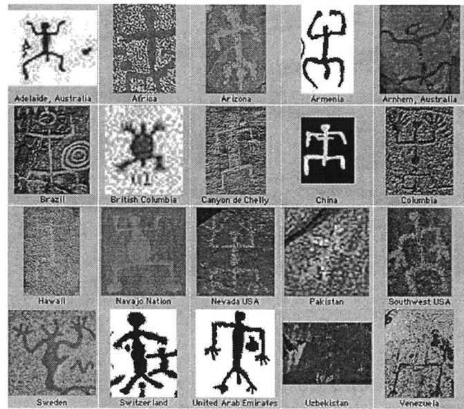
Fig. 30. Commonality of the most often depicted petroglyph, the squatter human or anthromorph.
