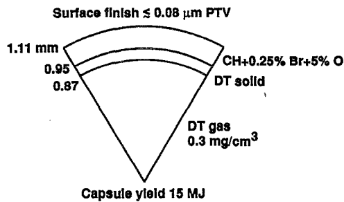
FIG. 106. Most of our modeling has concentrated on a 300 eV target, which absorbs 1.35 MJ of light.
