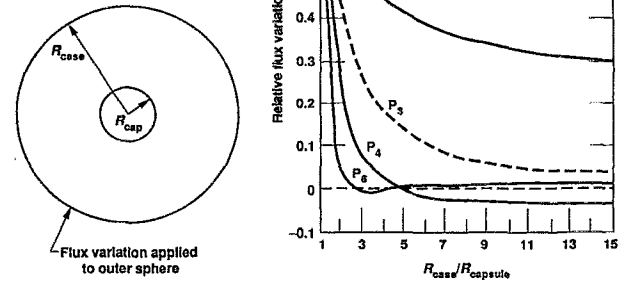
FIG. 61. Hohlraums with R_{\text{wall}}/R_{\text{capsule}} from about 3–5 effectively smooth all but the P_2 Legendre polynomial flux variations.
