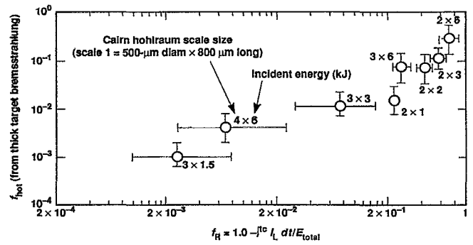
FIG. 21. The experimental hot-electron fraction f_{\text{hot}} in 1.06 μm hohlraum scales with the fraction of energy remaining in the pulse f_r at time t_c when the average hohlraum density reaches quarter-critical.
