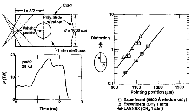
FIG. 75. Symmetry experiments with gas-filled hohlraums show the same variations with pointing position as empty hohlraums, but the data are offset from the current LASNEX calculations by 150 μm.
