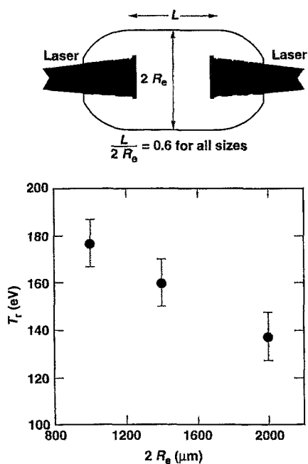
FIG. 11. Hohlraum drive on the Phebus laser 28 has been measured at 0.35 \mu\text{m} , E_{\text{laser}}=6 kJ in 1.3 ns, as a function of cavity diameter.
