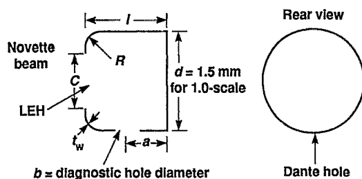
FIG. 32. Half-Cairn targets for Novette scaling experiments. Dimensions: d = outside diameter of cylinder = 1500 \mu\text{m} for 1.0 scale; l = length of cylinder = (5/6)d ; a = distance from back wall to center of Dante hole = (13/30)d ; b = diameter of Dante hole = (4/15)d ; c = LEH diameter = 0.5d ; t_w = wall thickness; R = radius of front corner = 0.25d ; g = back corner angle = 90 \pm 2^\circ .
