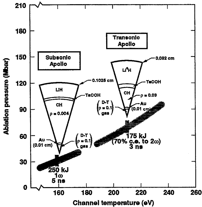
FIG. 26. Calculations in 1979, which predicted ignition for a 20-beam "200 kJ Nova," required high hohlraum coupling efficiency and near 1-D performance of double-shell targets. Both capsules had E_{\text{cap}} = 50 kJ, V(\text{TaCOH}) = 2 \times 10^7 cm/s, V(\text{Au}) = 3 \times 10^7 cm/s. Capsule yields were about 100 kJ.
