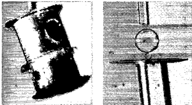
FIG. 13. The first indirect-drive, laser-driven implosion was achieved on the Cyclops laser at LLNL in 1976 using a target called a Forerunner.
