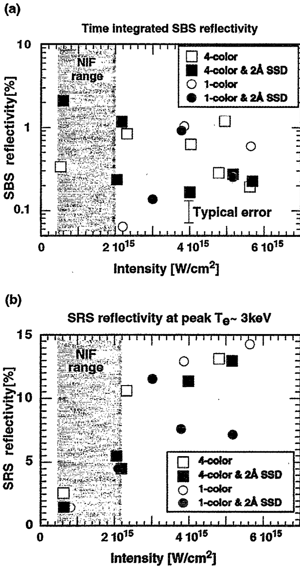
FIG. 101. (a) Time-integrated SBS reflectivities are 1% or less in energy from C_3H_{12} plasmas for both open (gasbag) and closed (hohlraum) geometries with f/8 focusing. Shown is the gasbag data. (b) For the range of intensities of interest to NIF ignition designs, SRS scattering levels are 2%–5% with phase plates and 2 Å of SSD. Without SSD temporal smoothing, the SRS level is about 10% at the upper end of the NIF intensity range, but still only about 2% at the lower end.
