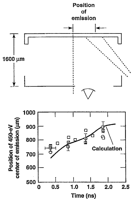
FIG. 77. The observed axial motion of the centroid of emission for ps22 is close to that calculated. In calculations, Nova beams are assumed to have a Gaussian profile, whereas the actual beam has significant structure, which makes identification of the beam centroid ambiguous. 96
