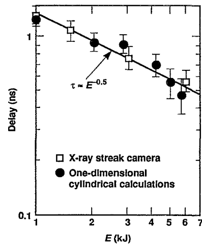
FIG. 22. High-energy electron time delay versus energy for Shiva 2.0-scale Cairn target (1000 μm diam by 1600 μm long) hohlraum (2 ns pulse).
