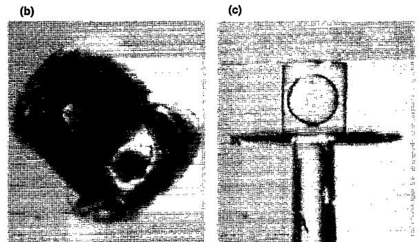
FIG. 14. Improved version of Forerunner target: (a) engineering drawing, (b) assembled target, and (c) fuel capsule and Parylene cover mounted on end cap prior to assembly.
