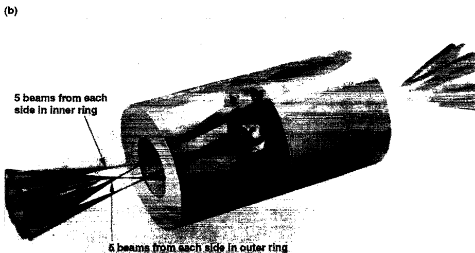
FIG. 18. (a) Cairn Mod-B, one of a series of targets that use radiation-driven, ablative compression of the fuel capsule. (b) Mod-B irradiation geometry for 20-beam Shiva laser.
