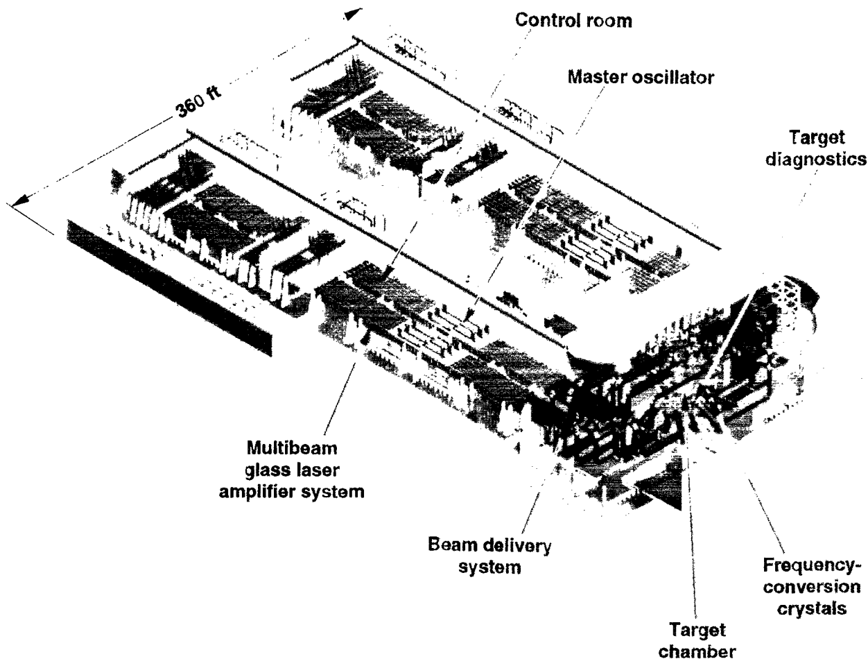
FIG. 104. The NIF is being designed to produce 1.8 MJ of 0.35 \mu\text{m} laser light with 500 TW for defense applications and inertial fusion ignition. The NIF will be able to explore ignition with both indirect-drive and direct-drive targets.
