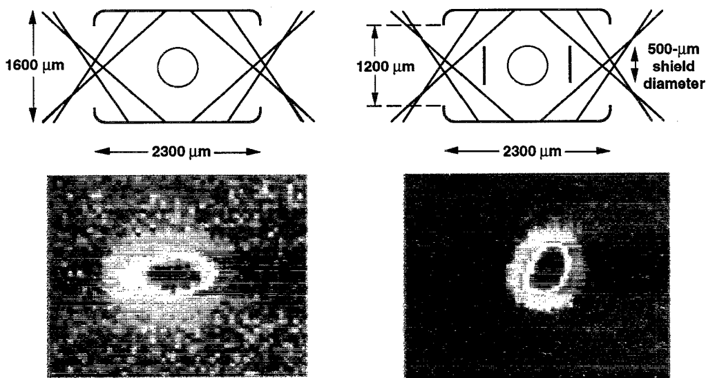
FIG. 78. Internal radiation shields modify implosion symmetry, in agreement with calculations.
