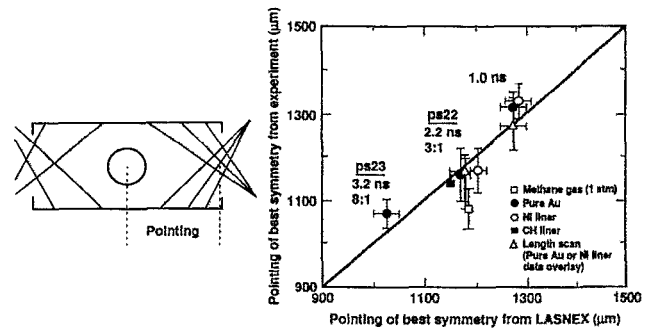
FIG. 76. LASNEX successfully predicts the pointing of best symmetry for almost all symmetry experiments. Beams must be moved inward for longer pulses to compensate for spot motion caused by hohlraum wall blowoff. The experimental pointing of best symmetry is offset from the calculations by \sim 150 \mu\text{m} for the methane-gas-filled hohlraums. The cause of this offset is being investigated.
