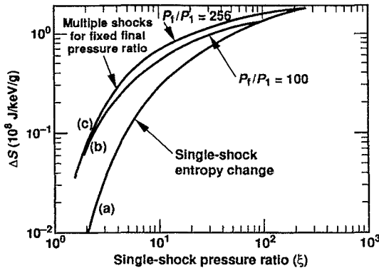
FIG. 38. Entropy changes in shocked DT: (a) for single shock; (b) multiple shocks versus individual shock pressure ratio with fixed final-to-initial pressure ratio P_f/P_1=100 ; (c) multiple shocks versus individual shock pressure ratio with P_f/P_1=256 .
