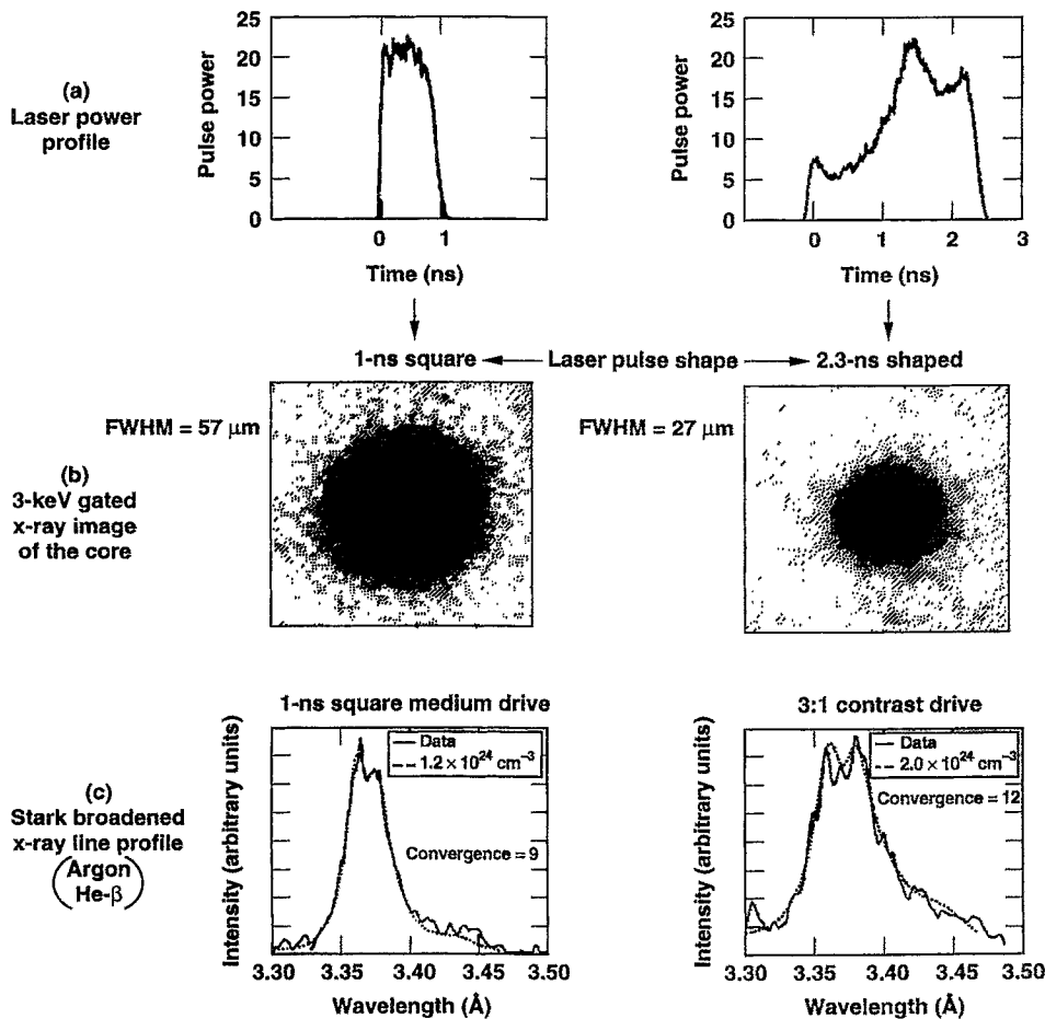
FIG. 41. Implosion experiments with shaped drive demonstrate higher convergences and fuel densities at the same peak drive pressure.
