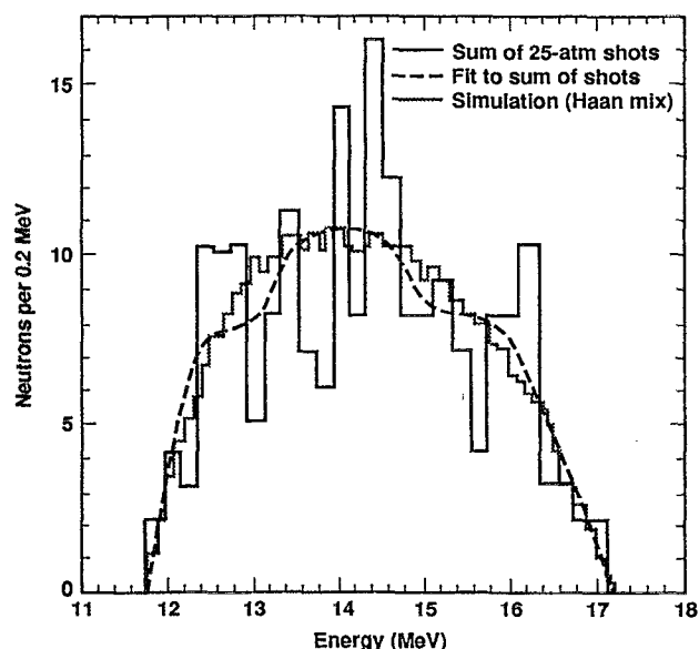
FIG. 87. Shape of composite neutron spectrum of 25 atm experiments (ten shots) is well modeled by simulation with the Haan mix model. 204
