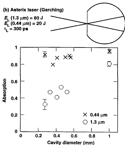
FIG. 28. Small-target hohlraum experiments showed efficient coupling with short-wavelength laser light. (a) Results from 1981 Argus laser experiments at LLNL using 0.35, 0.53, and 1.06 \mu\text{m} light. (b) Asterix laser (Garching, 1988) results using 0.44 and 1.3 \mu\text{m} light.
