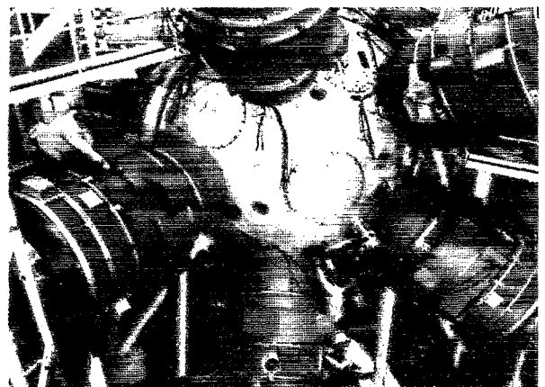
FIG. 9. Nova target chamber.
