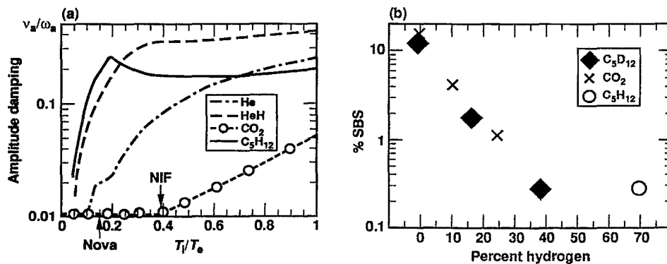
FIG. 91. Damping rates for helium-hydrogen mixtures in NIF are larger than for Nova CH mixtures: (a) 50/50 mixture of helium and hydrogen consistent with a 17 K cryogenic target; (b) protons mixed with CO 2 or C 5 D 12 reduced reflectivity in Nova experiments.
