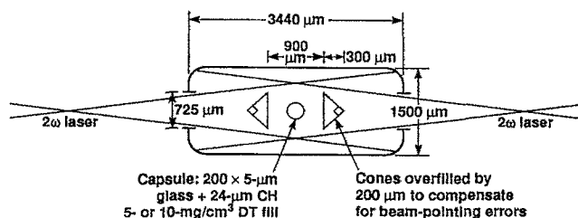
FIG. 30. Laser-target configuration for the two-beam Novette laser implosion campaign in 1983. These dimensions define a scale-1 Novette target.
