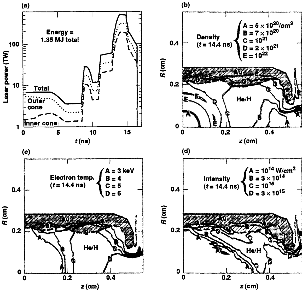
FIG. 90. Ignition-scale hohlraums at peak power have large regions in the laser channel with n/n_c \approx 0.1 and T_e \approx 4-6 keV.
