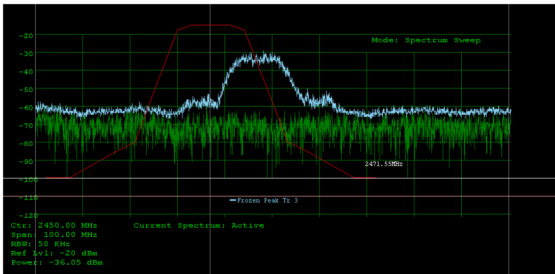
Fig. 11. MAX2820 receiver filter's frequency response on channel 6 (red) and signal trace on channel 8 (blue).
