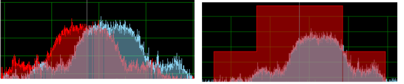
(a) Two DSSS signals shown together. The receiver filter may be estimated using a transmission on the receiver's channel (channel 6 here, shown in red). The blue trace belongs to an interferer on the adjacent channel 7. (b) The receiver filter, in red, estimated as the DSSS TSM centered on channel 6 and the captured interferer DSSS signal, in blue, on channel 7, shown together.
