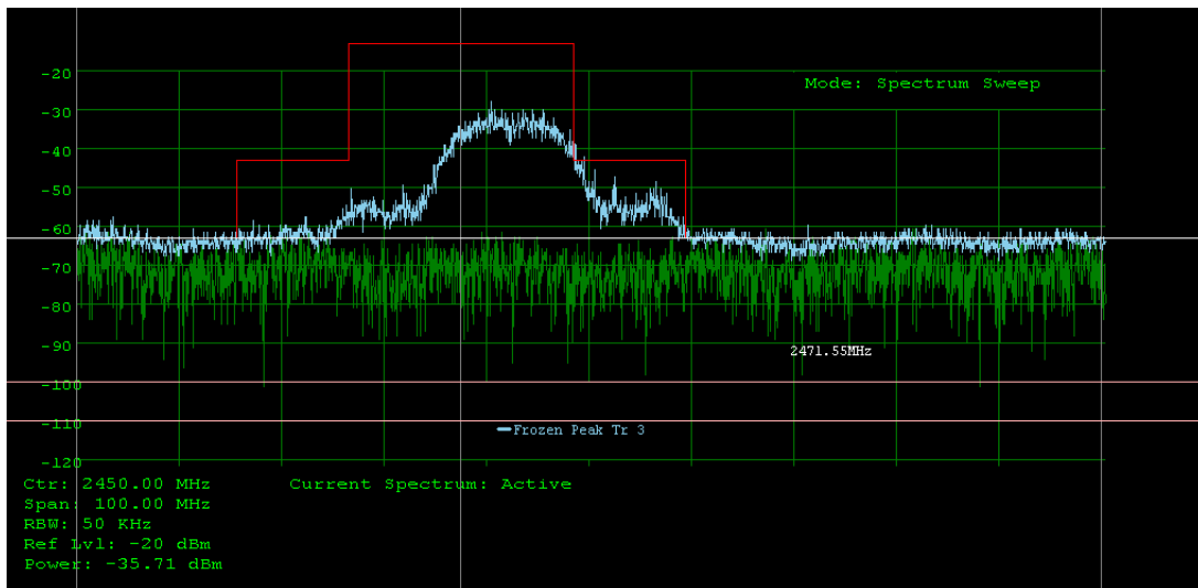
Fig. 6. TSM on channel 6 (red) and signal trace on channel 7 (blue).
