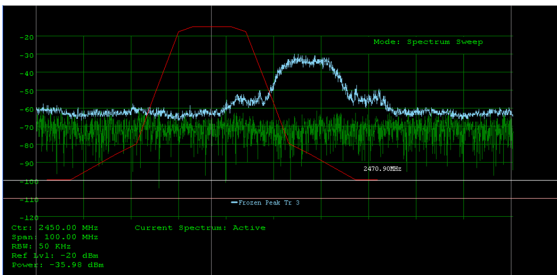
Fig. 12. MAX2820 receiver filter's frequency response on channel 6 (red) and signal trace on channel 10 (blue).
