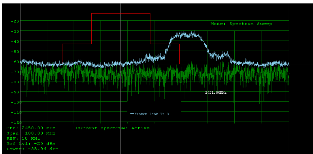
Fig. 8. TSM on channel 6 (red) and signal trace on channel 11 (blue).
