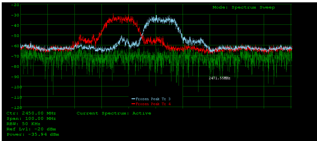
Fig. 4. Signal traces showing overlap between transmitted signals on channels 6 (red trace) and 9 (blue trace).
