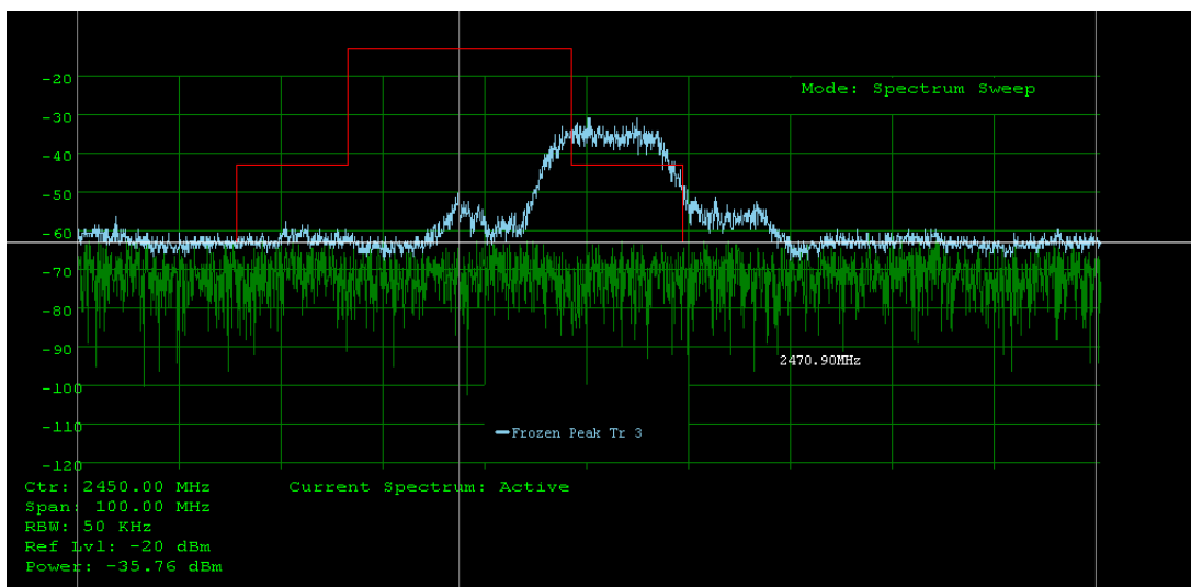
Fig. 7. TSM on channel 6 (red) and signal trace on channel 9 (blue).
