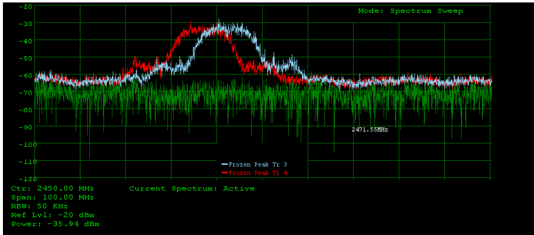
Fig. 3. Signal traces showing overlap between transmitted signals on channels 6 (red trace) and 7 (blue trace).
