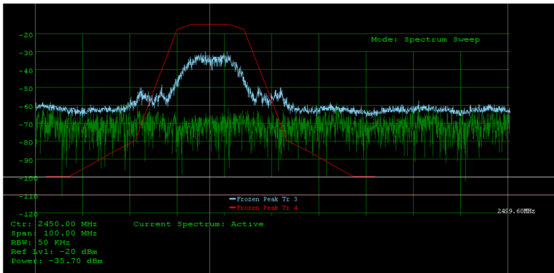
Fig. 10. MAX2820 receiver filter's frequency response on channel 6 (red) and signal trace on channel 6 (blue).
