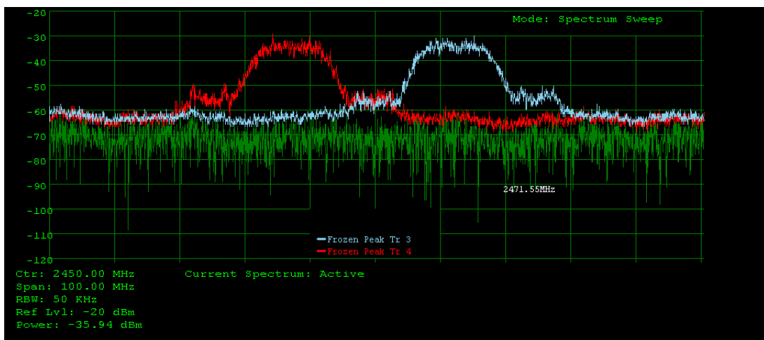
Fig. 5. Signal traces showing overlap between transmitted signals on channels 6 (red trace) and 11 (blue trace).
