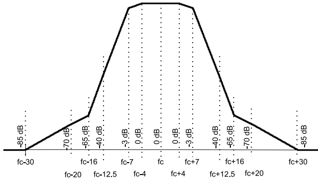
Fig. 9. Receiver filter's frequency response of the Maxim MAX2820/MAX2821 802.11b transceiver. f_c denotes the center frequency, and the unit of the x -axis is MHz.
