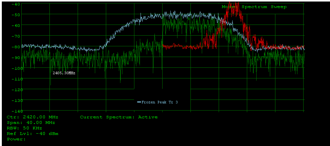
Fig. 16. Signal traces showing overlap between 802.11 channel 3 (blue) and 802.15.4 channel 16 (red).
