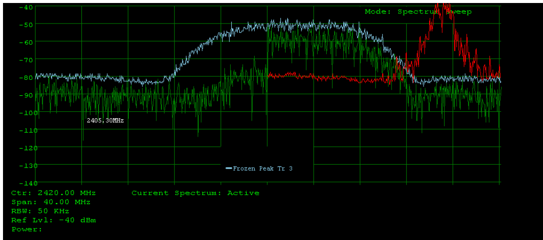
Fig. 17. Signal traces showing overlap between 802.11 channel 3 (blue) and 802.15.4 channel 17 (red).
