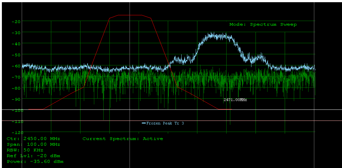
Fig. 13. MAX2820 receiver filter's frequency response on channel 6 (red) and signal trace on channel 12 (blue).
