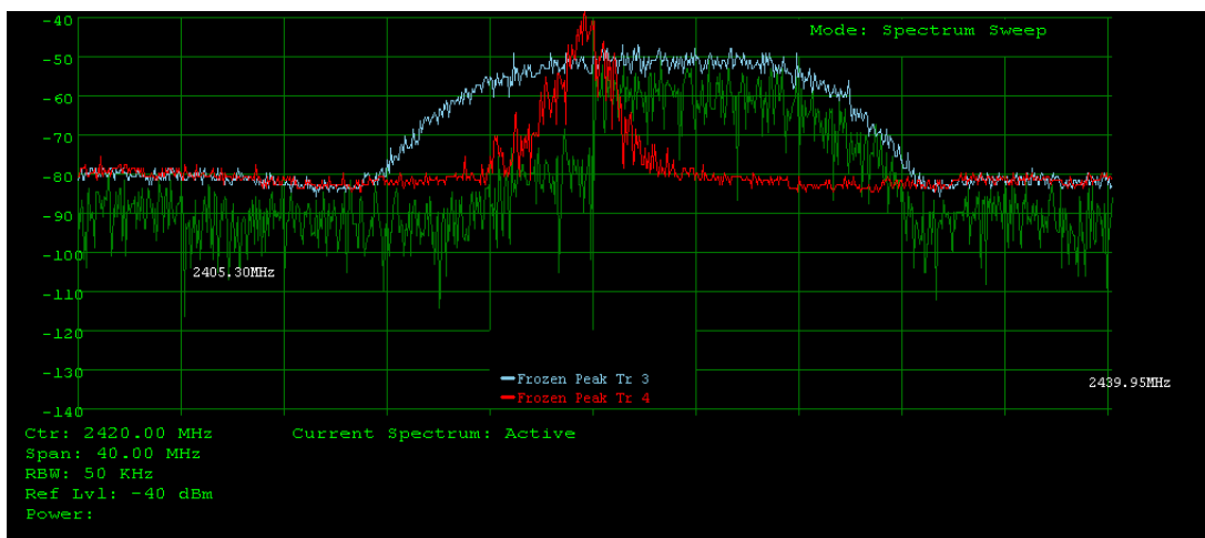
Fig. 15. Signal traces showing overlap between 802.11 channel 3 (blue) and 802.15.4 channel 14 (red).
