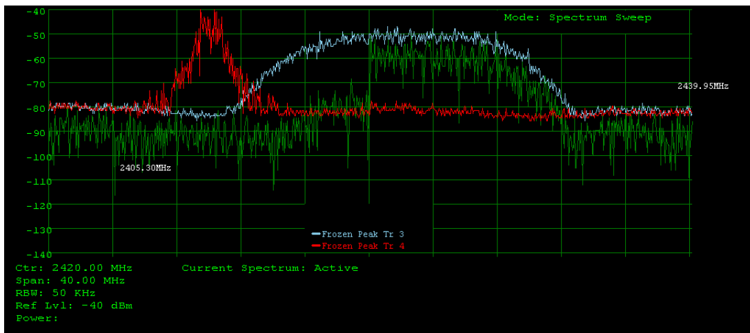
Fig. 14. Signal traces showing overlap between 802.11 channel 3 (blue) and 802.15.4 channel 12 (red).
