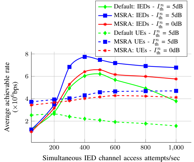
Fig. 3. Average achievable rates for cellular UEs and D2D-capable IEDs in the default transmission case and with the proposed MSRA scheme for different interference tolerance levels with given p_{c,\text{th}} = 10^{-3} and increasing IED traffic load.
