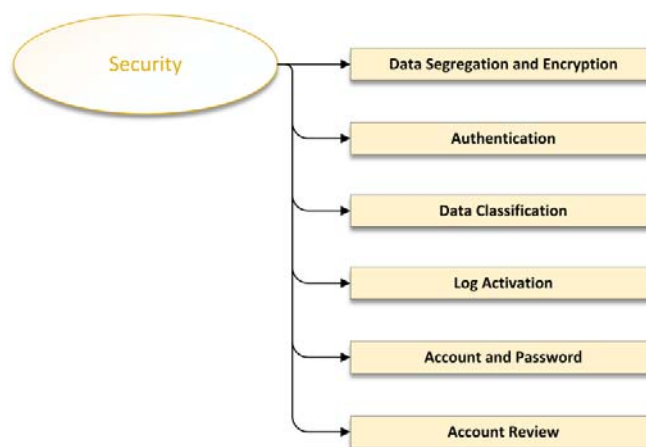
Fig. 9 Security Indicators
