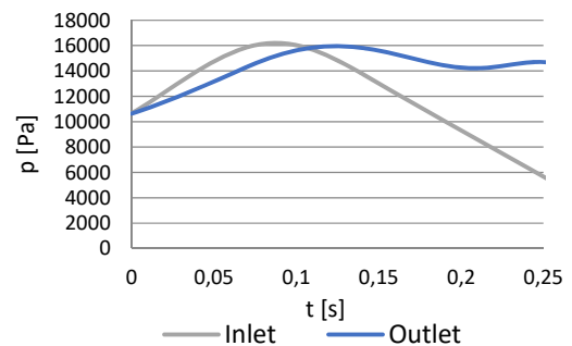
Fig. 6 Pressure boundary conditions
