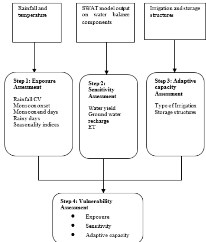
Fig. 2 Vulnerability assessment: A 4-step approach
