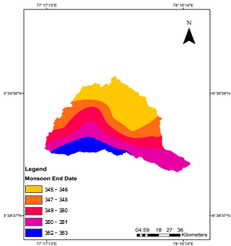
Fig. 3 (c) Spatial mapping of Monsoon End Date
