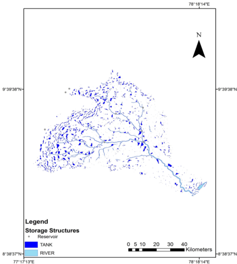
Fig. 5 (b) Spatial mapping of Storage structures
