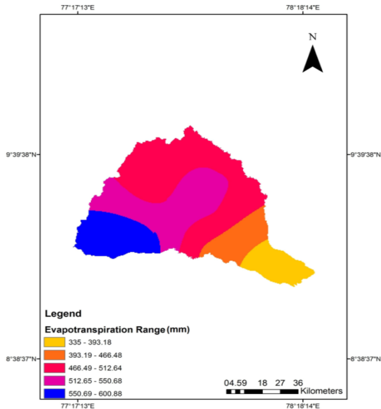
Fig. 4 (c) Spatial mapping of Evapotranspiration
