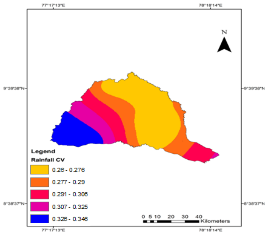
Fig. 3 (a) Spatial mapping of Rainfall CV
