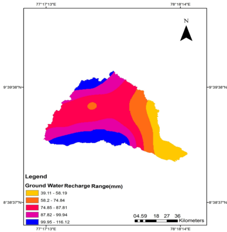
Fig. 4 (b) Spatial mapping of Ground water recharge
