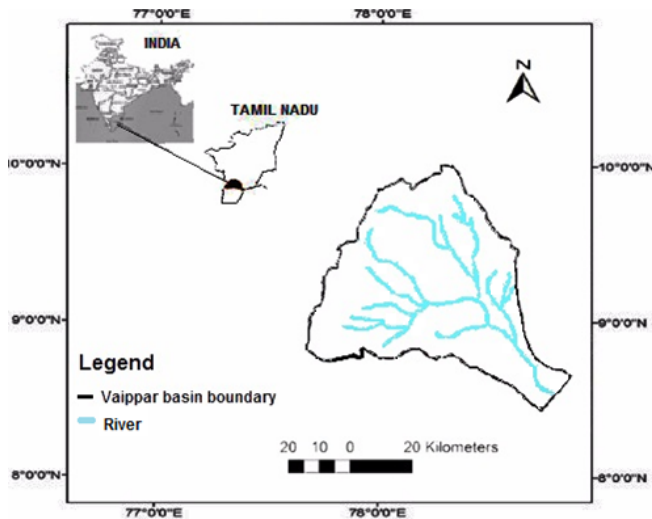
Fig. 1 Index map of the Vaippar basin
