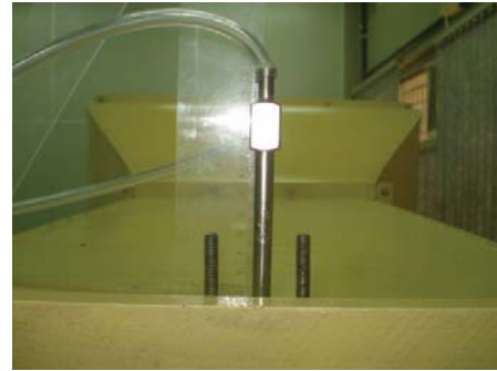
Fig. 4 Height adjustment of the Pitot tube
