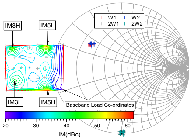
Fig. 10 Experimentally measured IM linearity contours as a function of IF reflection coefficient ( \Gamma_L ) for a class-J emulated RF impedance environment
