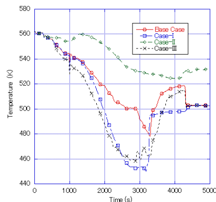
Fig. 8 Cold-Leg Fluid Temperatures in Broken Loop
