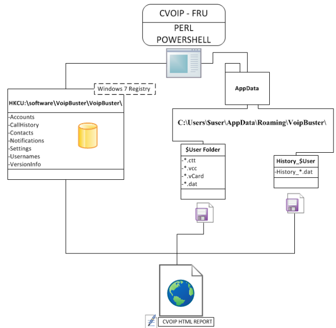
Fig. 2 CVOIP-FRU Detailed Windows Scripting Architecture
