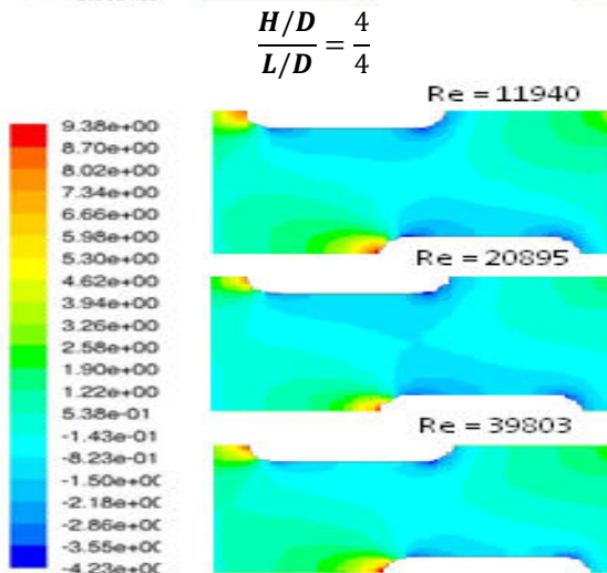
Fig. 3 Pressure drop contour for turbulent flow with Re number for different aspect ratio ( \frac{H/D}{L/D} )
