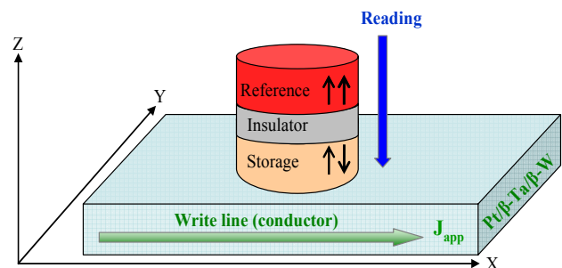
Fig. 2 Schematic of the three-terminal SOT device and the two independent paths for read and write operations. In-plane current injection through the write line (conductor) induces the perpendicular switching of the storage layer
