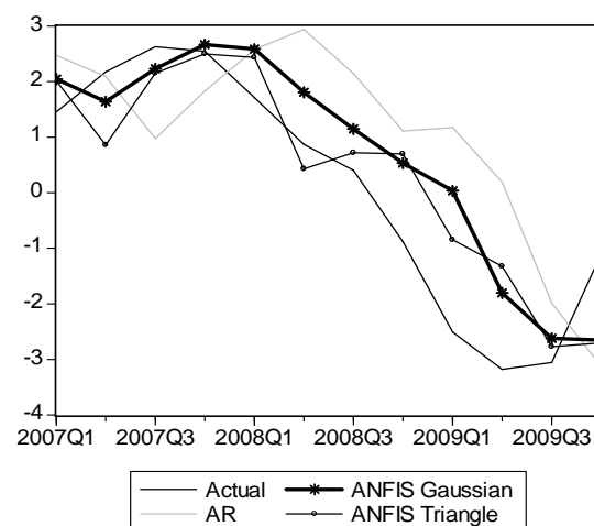
Fig. 3. Out-of-sample period forecasts with AR and ANFIS for France
