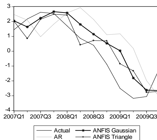
Fig. 2. Out-of-sample period forecasts with AR and ANFIS for Canada
