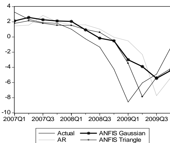
Fig. 5. Out-of-sample period forecasts with AR and ANFIS for Japan
