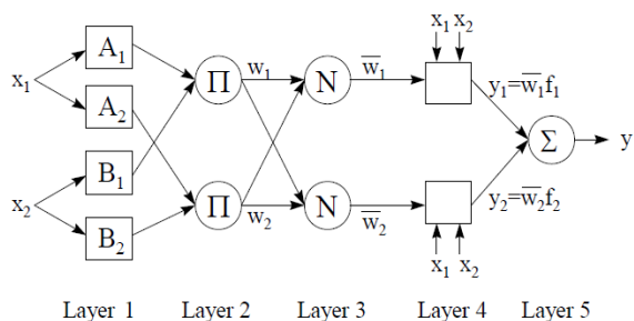
Fig. 1. Example of ANFIS architecture for a two-input, two-rule first-order Sugeno model
