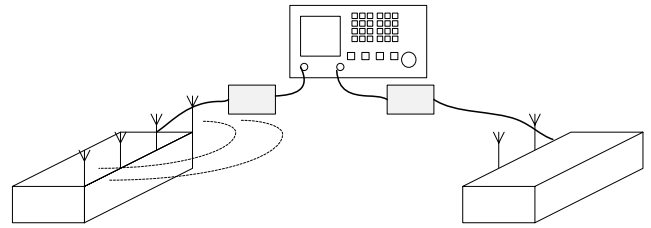
Fig. 2 Measurement set up.
