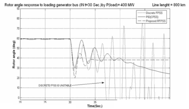
Fig. 11-d P(Load) = 400 MW
