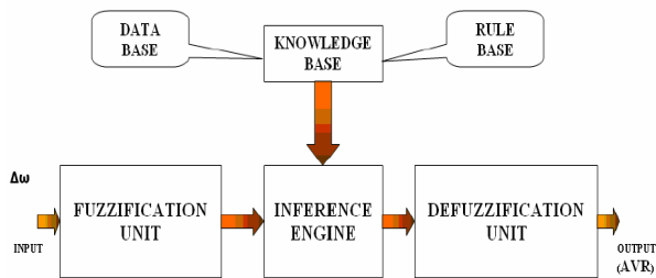
Fig. 3 Model of fuzzy controller and its blocks
