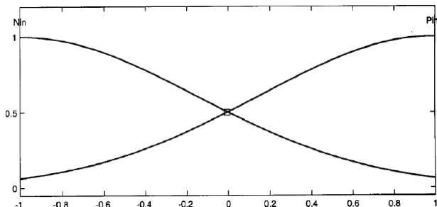
Fig. 4 Input membership functions
