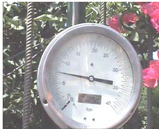
Fig. 5 Displaying the amount of force required to pull out the pile.
