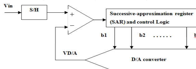
Fig. 2 SAR architecture
