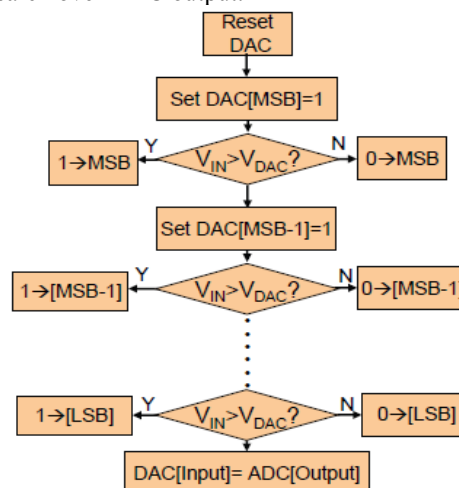
Fig. 1 SAR ADC algorithm block diagram [4]
