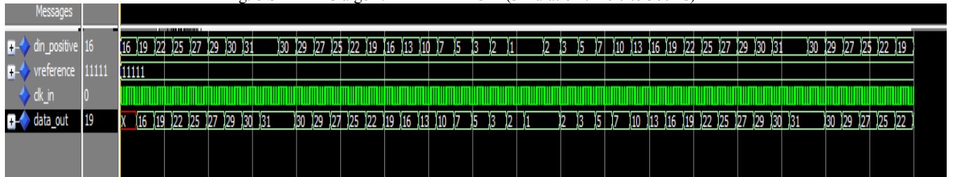
Fig. 9 SAR ADC algorithm in modelsim (simulation time 0 to 360 ns)
