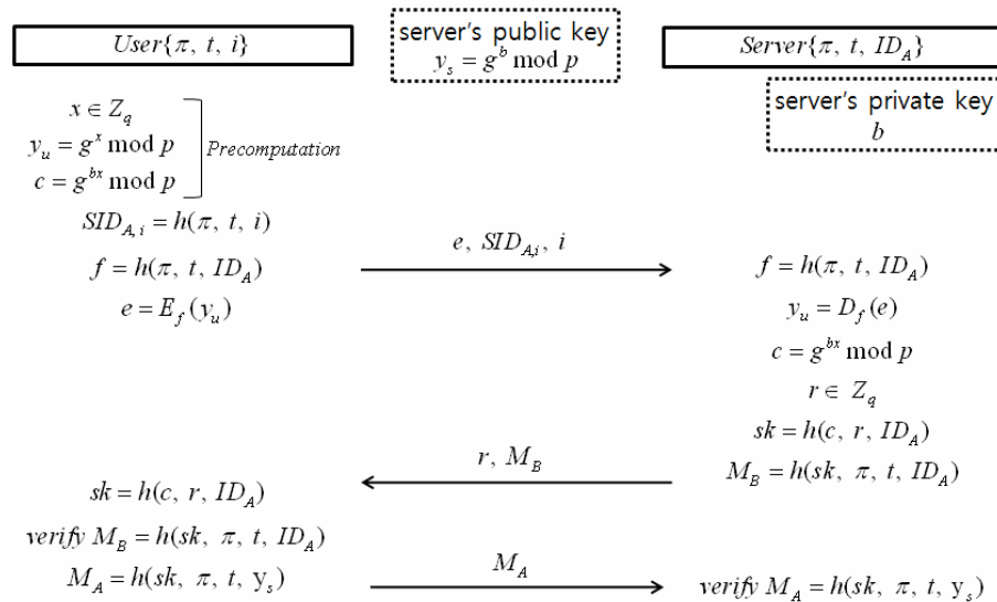
Fig. 2 A Protocol Proposed by Juang et al.
