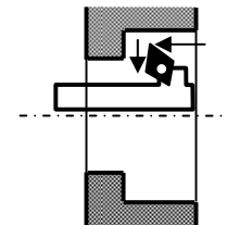
(b) Internal Step Turning
