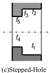
Fig. 21 Features extracted by the Extended SRG Method
